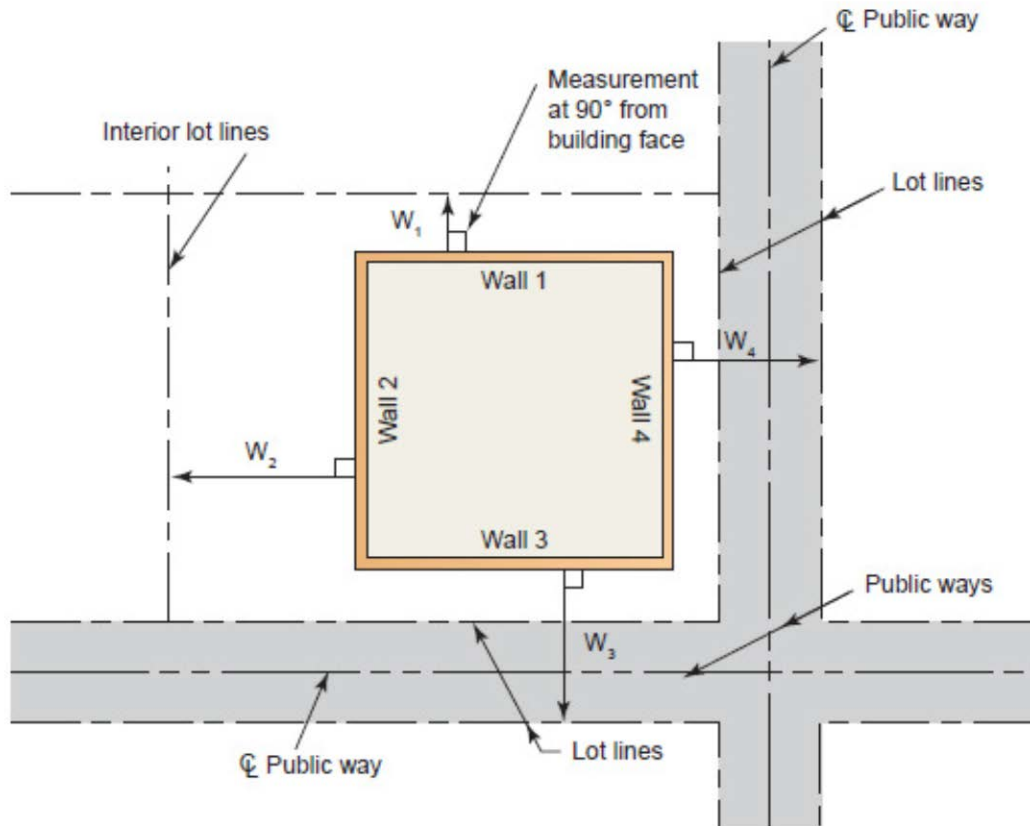
Allowable area frontage increase
