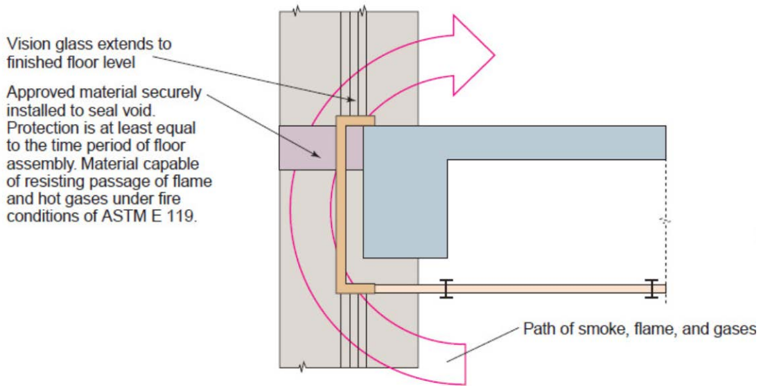
Joint protection at exterior curtain wall/floor intersection
