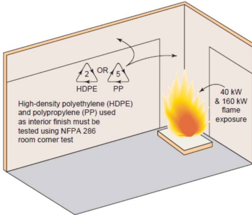
Room corner test
