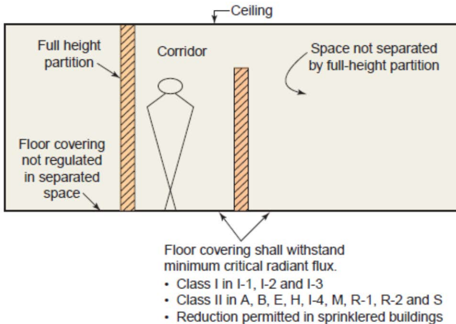
Interior floor finish requirements
