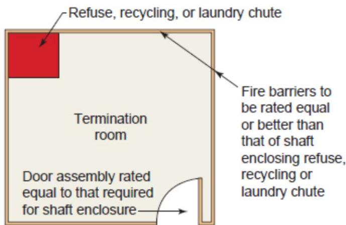
Refuse chute termination room
