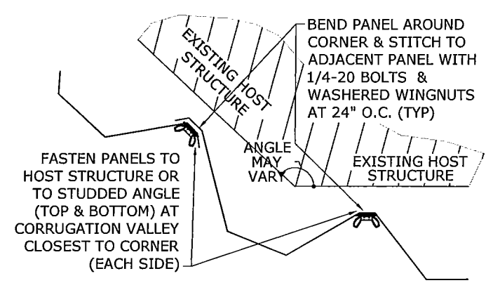
5 CORNER CLOSURE 3" = 1'-0" PLAN VIEW
