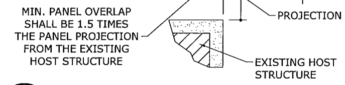
9 PANEL OVERLAP 3" = 1'-0" PLAN VIEW
