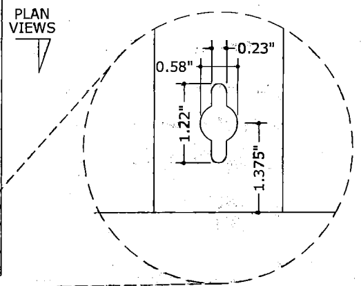
2 KEYHOLE DETAIL 1 N.T.S. ALT: FIELD DRILL \varnothing 3/8" HOLE (OR \varnothing 5/8" HOLE W/ KEYHOLE WASHER)
