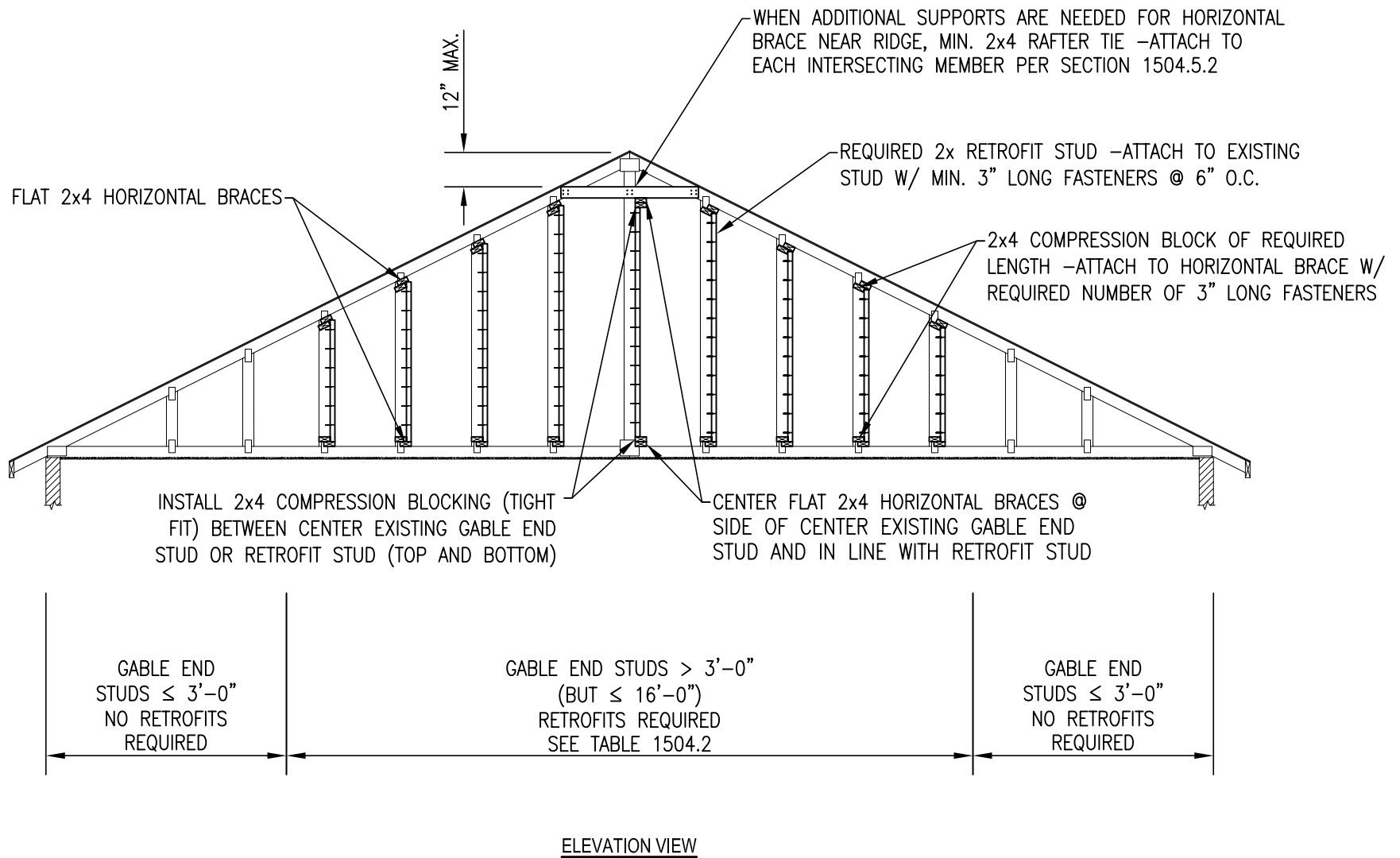
FIGURE 1504.5.2 DETAIL OF RETROFIT RIDGE TIE INSTALLATION
