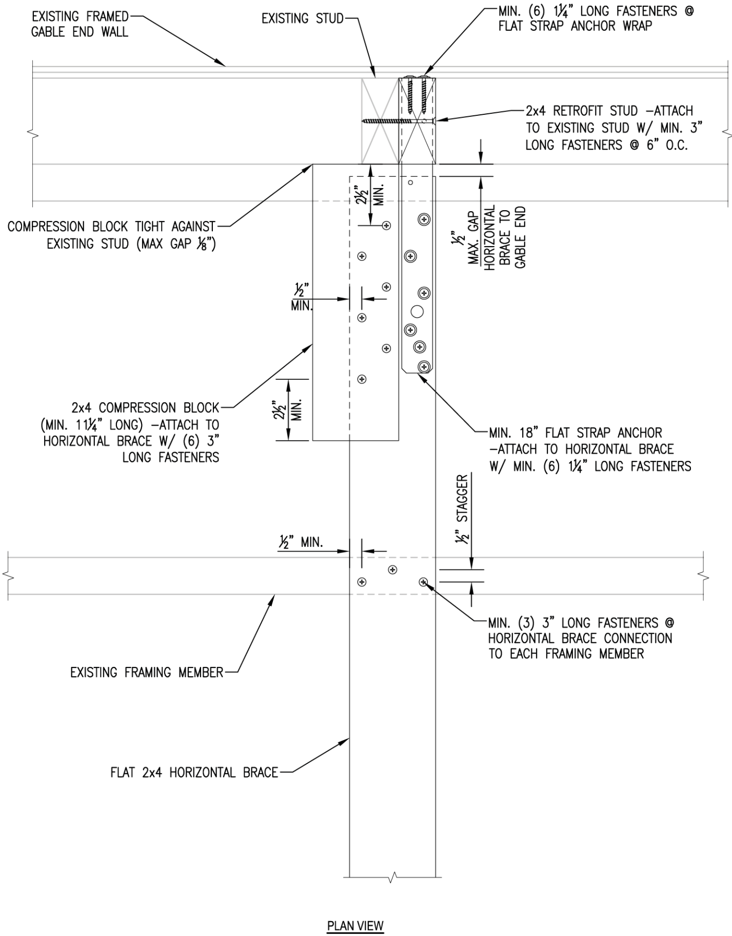
FIGURE A104.2.7 DETAILS OF STRAP & COMPRESSION BLOCK INSTALLATION - 2x4 RETROFIT STUD
