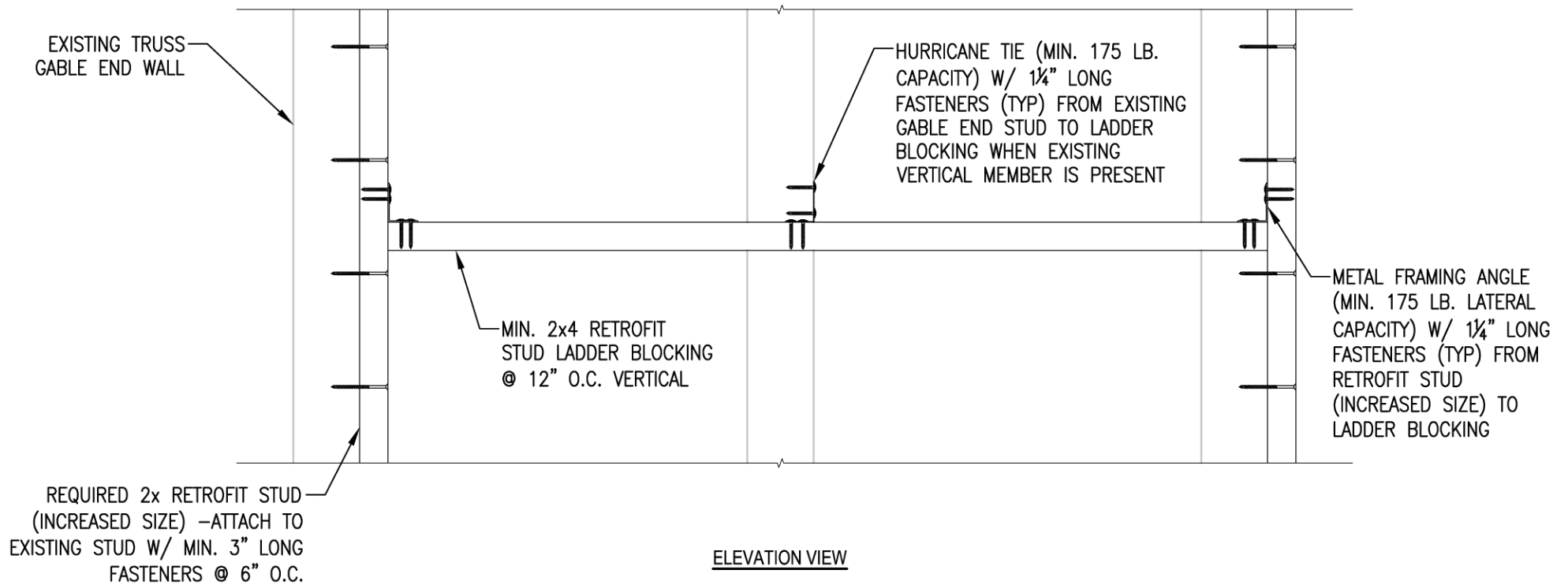
FIGURE A104.5.1.1 DETAIL OF LADDER BRACING FOR OMITTED RETROFIT STUD (TRUSS GABLE END)
