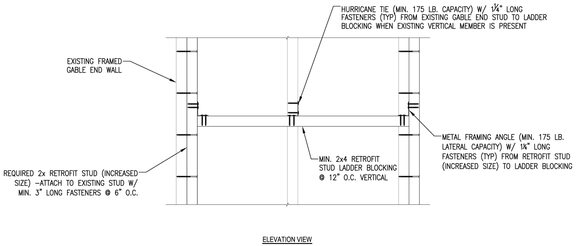
FIGURE A104.5.1.2 DETAIL OF LADDER BRACING FOR OMITTED RETROFIT STUD (CONVENTIONAL FRAMING)
