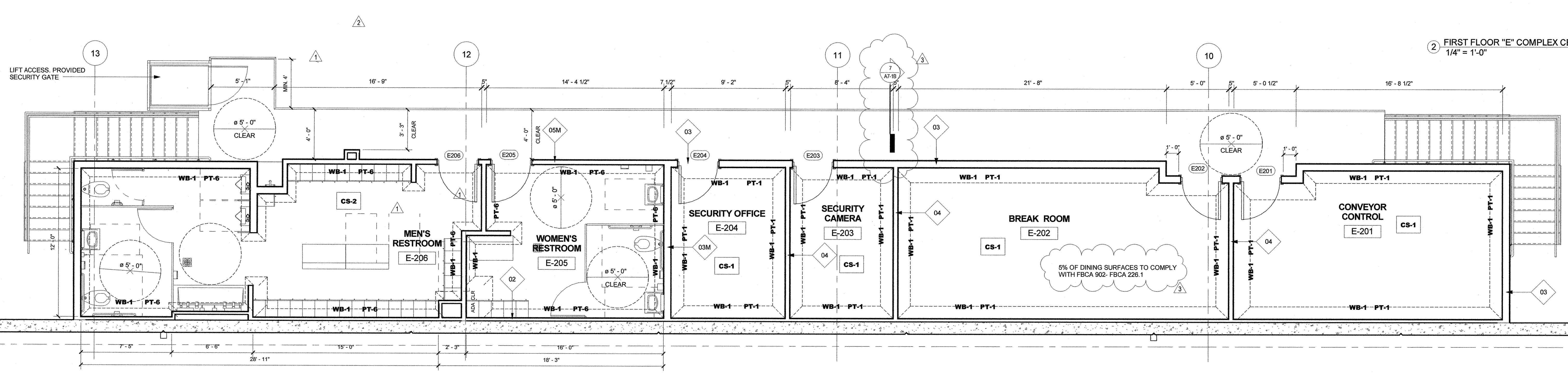
3 MEZZANINE FLOOR "E" COMPLEX 1/4" = 1'-0"
