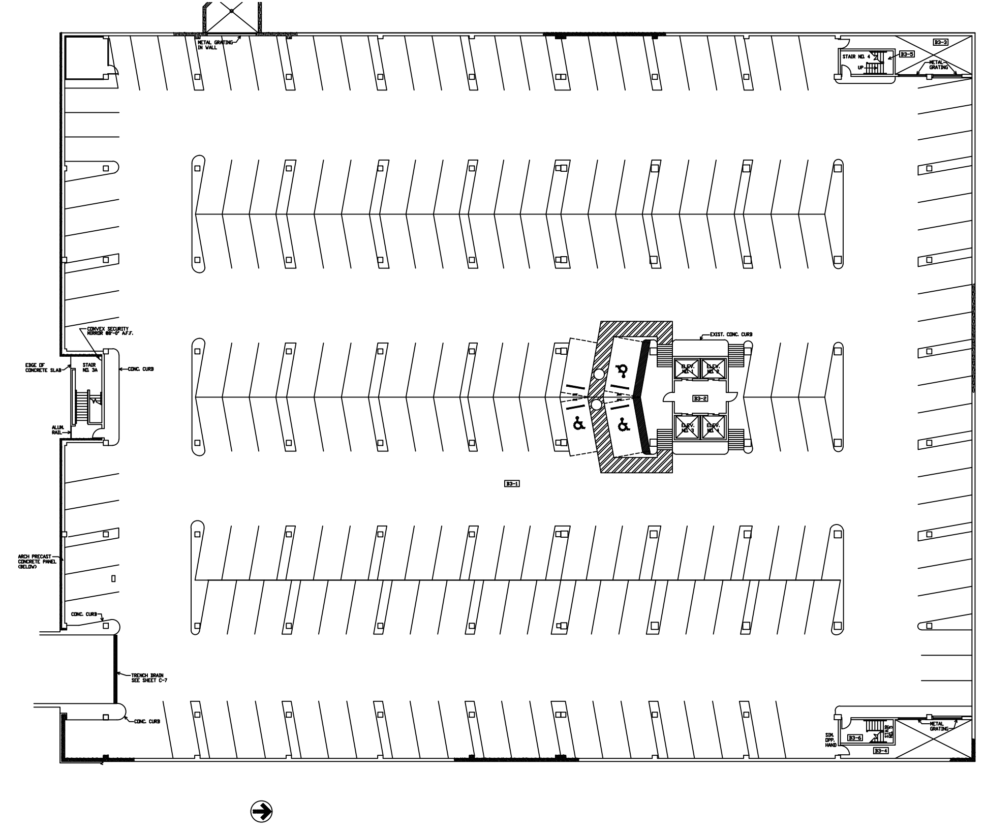
1 PARKING DECK LEVEL 3 SCALE 1/32"=1'-0"
