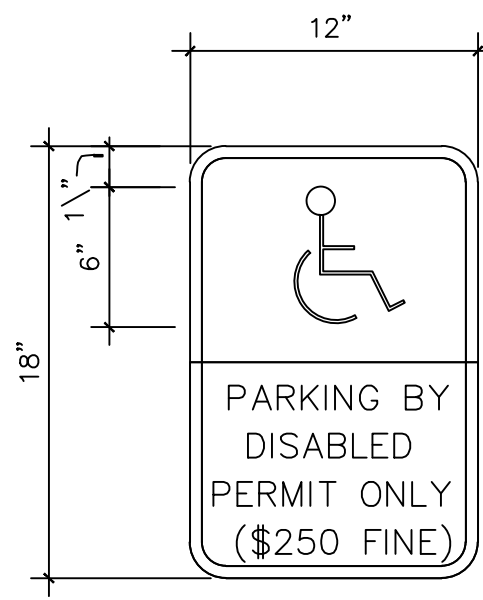
3 H/C PARKING SIGN NOT TO SCALE
