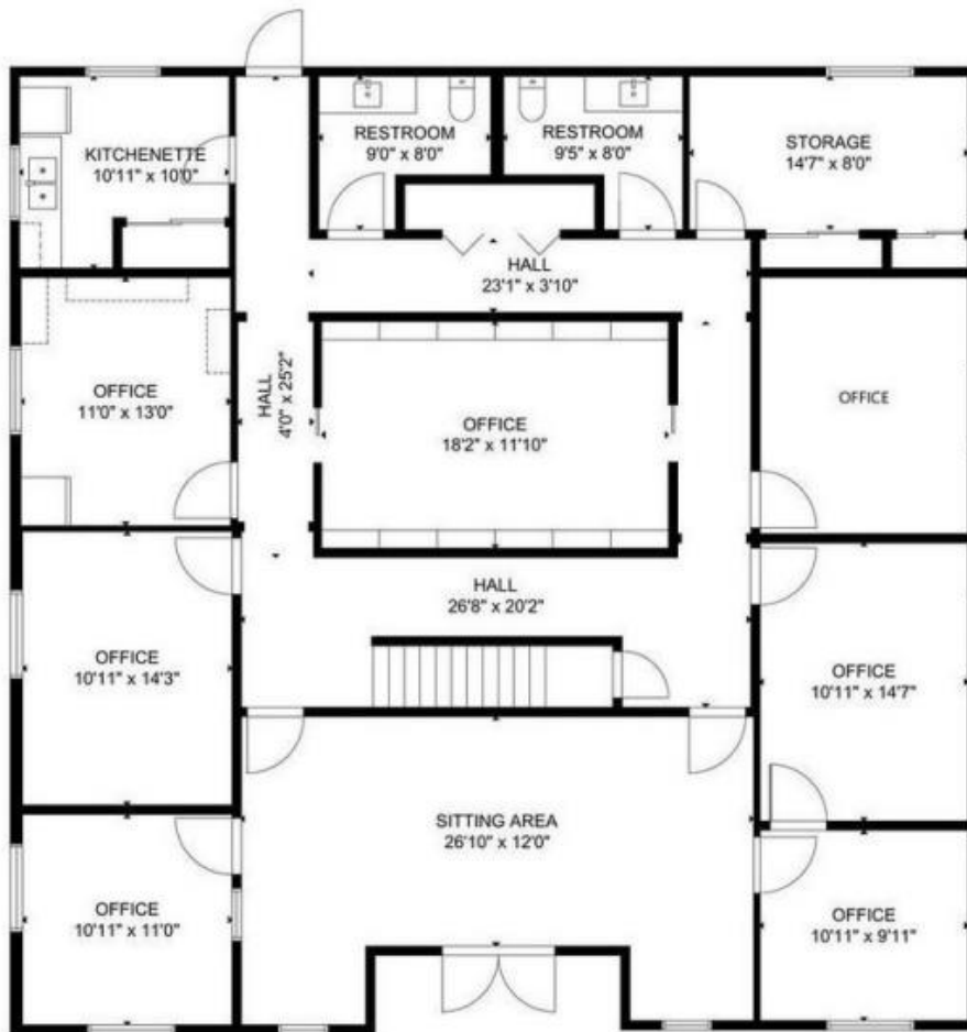
FLOOR 1
