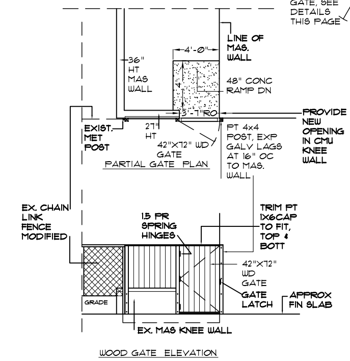
WOOD GATE ELEVATION
