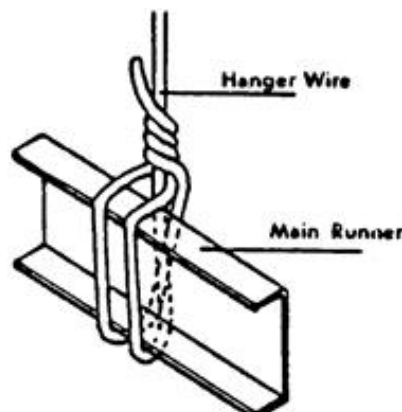
FIG. 1 Saddle Tie
