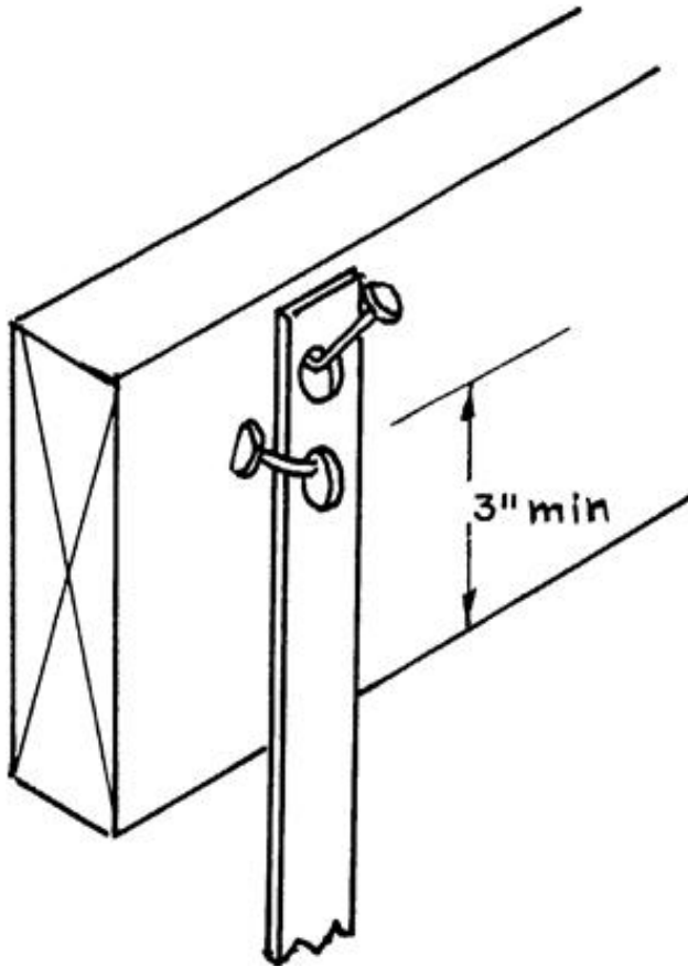
FIG. 7 Flat Hanger Attached to Support Using Nails
