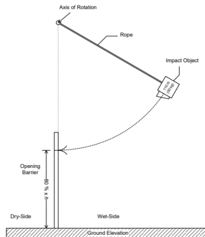
Figure 4.3.4 Impact Test Layout
