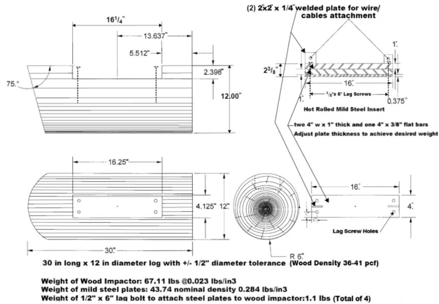
Fig. 2 (Impactor Design)
