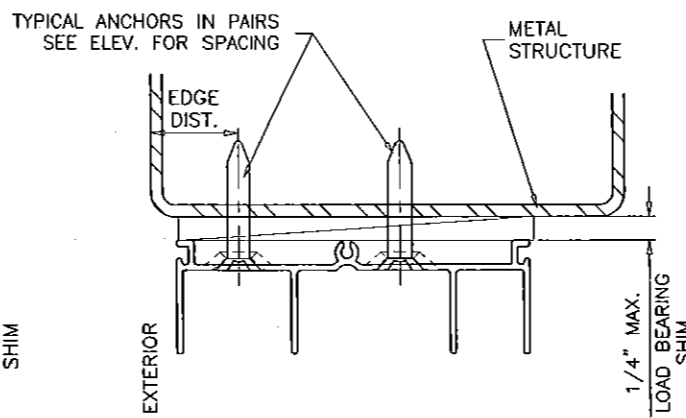
TYPICAL ANCHORS IN PAIRS SEE ELEV. FOR SPACING
