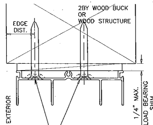
TYPICAL ANCHORS IN PAIRS SEE ELEV. FOR SPACING
