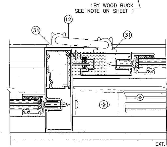
SECURITY LOCK AT ASTRAGAL STILE
