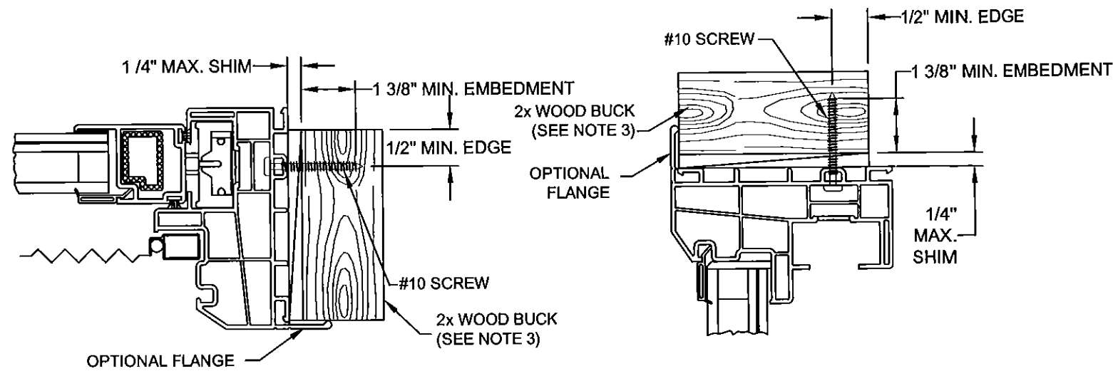
HEAD W/ BOX FRAME THROUGH FRAME INTO 2x WOOD
