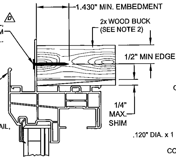
HEAD W/ NAIL FIN THRU NAIL FIN INTO WOOD FRAMING
