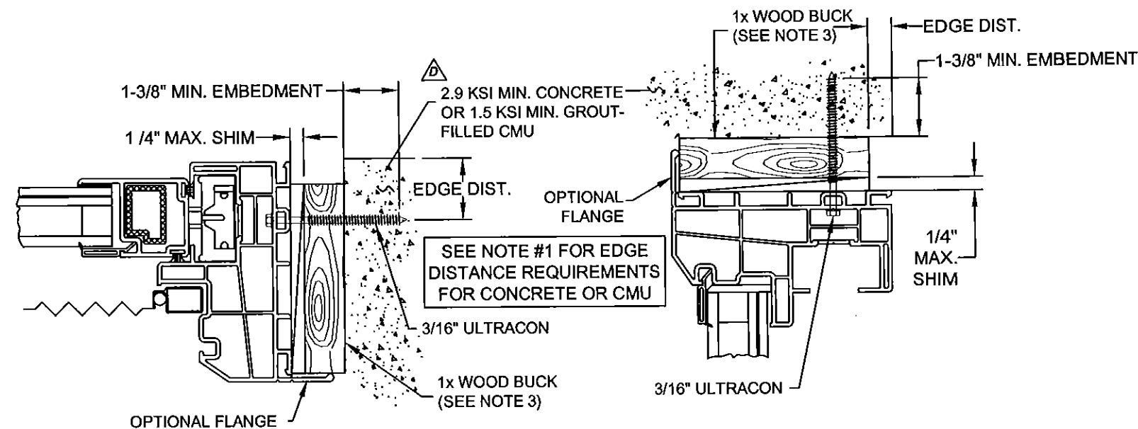
HEAD W/ BOX FRAME THROUGH FRAME INTO CONCRETE 1x BUCK OPTIONAL
