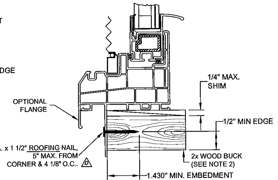
SILL W/ NAIL FIN THRU NAIL FIN INTO WOOD FRAMING
