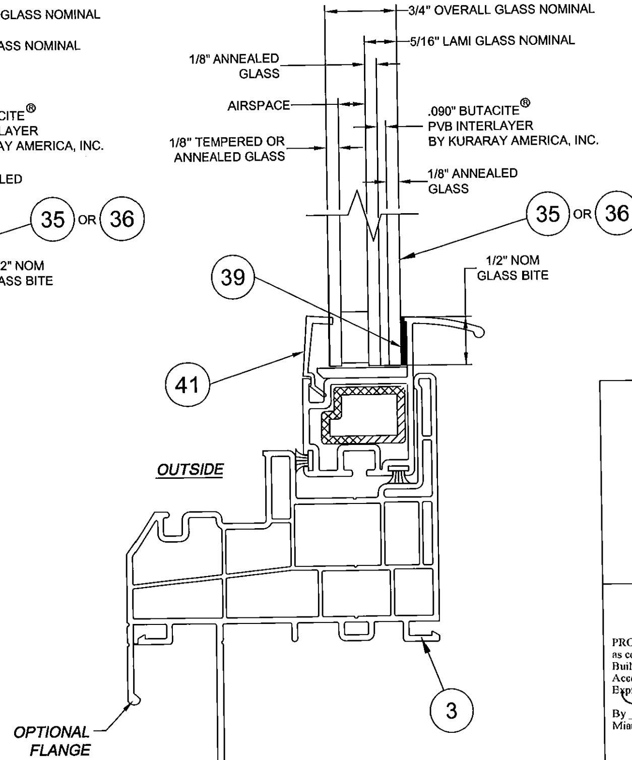
3/4" LAMI I.G. GLAZING DETAIL WITH 5/16" LAMI GLASS AND 1/8" CAP BOX OR INTEGRAL FIN FRAME (INTEGRAL FIN FRAME SHOWN)
