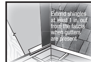
Figure 3L Valley/Shingle Extension
