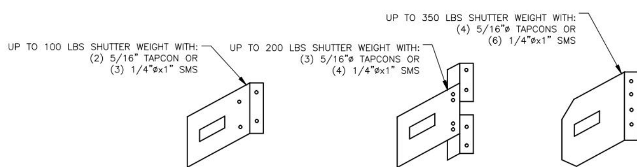
MOUNTING BRACKET END-RETENTION INSTALLATION - N.T.S.
