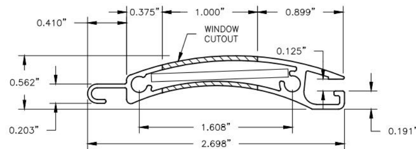
5050-H112 ALUMINUM 58MM SLAT SPANS UP TO 108" END-RETENTION VIEWPOINT SLAT - SCALE 1:1
