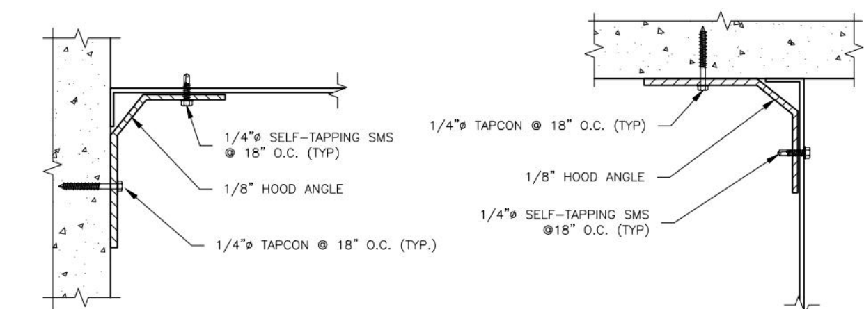
CUSTOM HOOD WALL ATTACHMENT END-RETENTION INSTALLATION - N.T.S.
