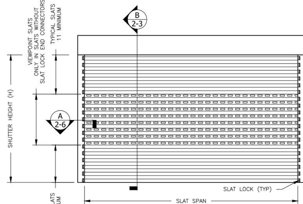
ALTERNATING VIEWPOINT UNIT ELEVATION SPANS UP TO 108" SINGLE OR MULTIPLE UNIT INSTALLATIONS - N.T.S.
