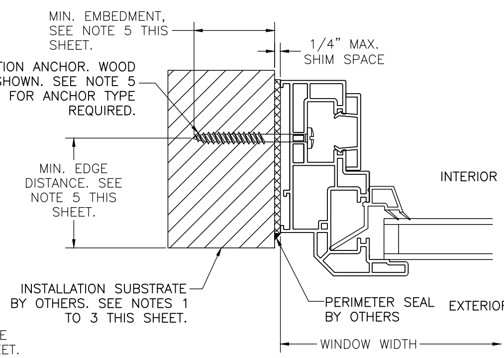
HORIZONTAL (JAMB) CROSS SECTION WOOD FRAMING, 2X WOOD BUCK, CONCRETE/MASONRY OR METAL FRAME APPROVED
