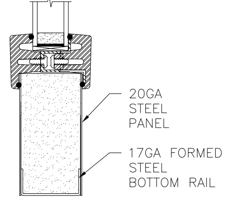
OPTION 9 SMOOTH TRIM
