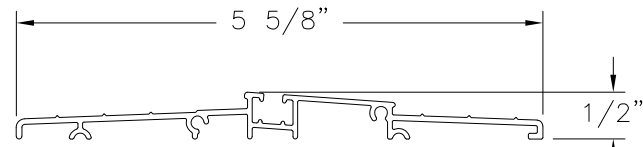
ADA OUTSWING THRESHOLD
