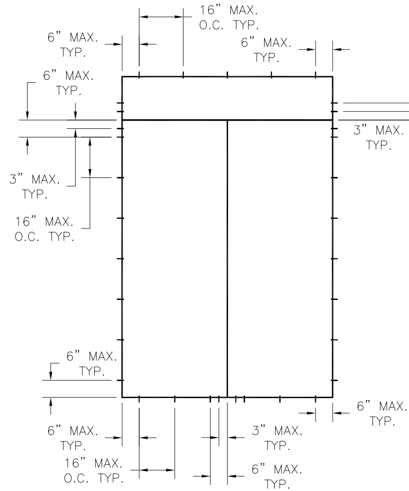
DOUBLE W/TRANSOM
