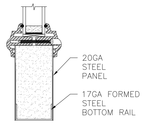
OPTION 10 EVOLVE TRIM
