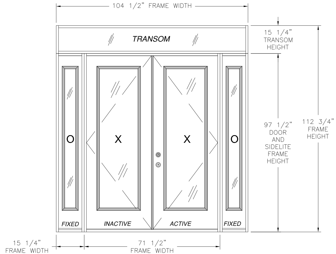
20GA STEEL OS DOUBLE DOOR W/ SIDELITES AND TRANSOM EXTERIOR VIEW
