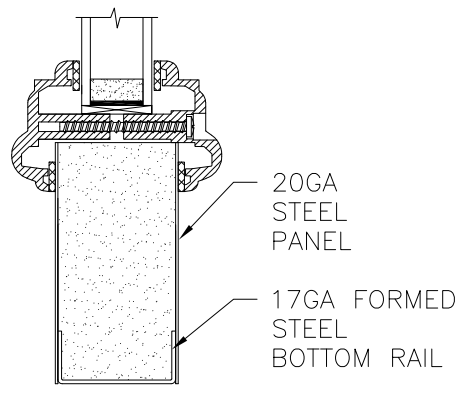
OPTION 23 ELTON TRIM
