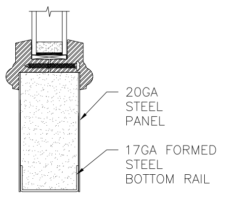
OPTION 12 RSL TRIM
