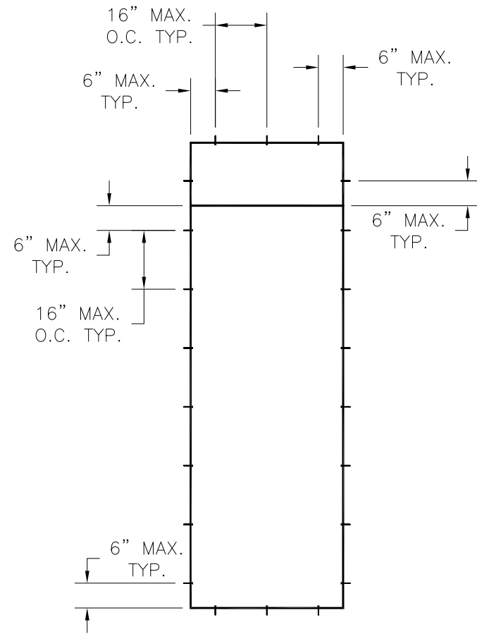
SINGLE W/TRANSOM
