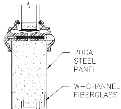
OPTION 16 EVOLVE TRIM
