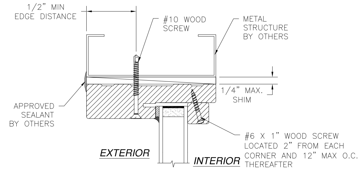
TRANSOM DETAIL INSWING/OUTSWING METAL STRUCTURE INSTALLATION HEAD SHOWN JAMBS SIMILAR
