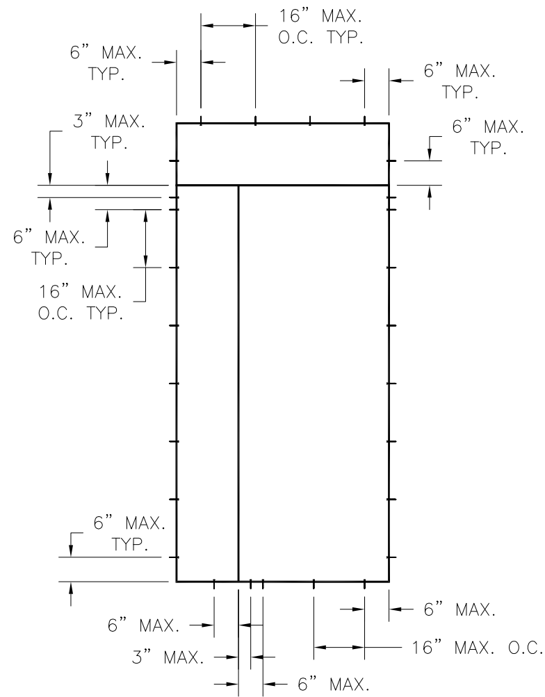
SINGLE W/SIDELITE & TRANSOM
