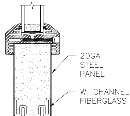
OPTION 17 SPOTLIGHT TRIM
