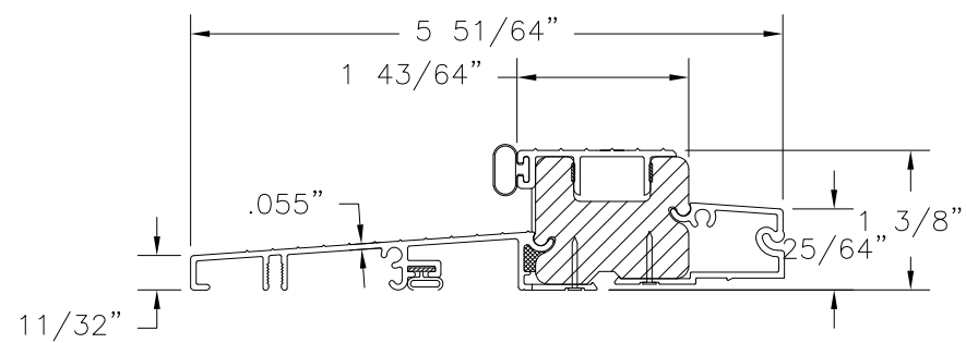
OUTSWING SILL
