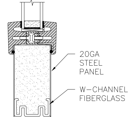
OPTION 27 SMOOTH TRIM W/TAPE
