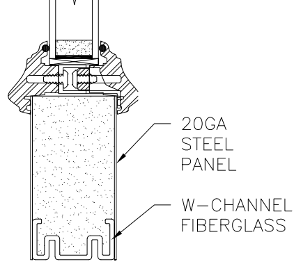
OPTION 14 SIGNET TRIM
