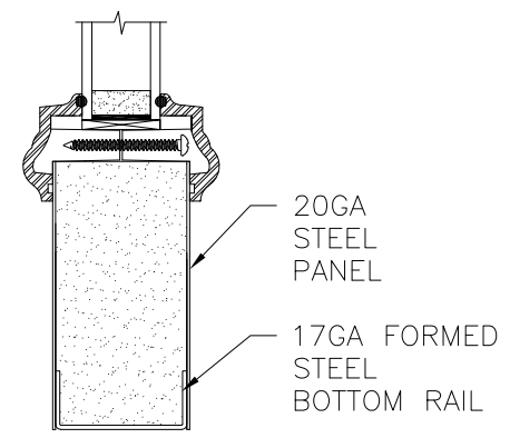
OPTION 7 TRINITY TRIM
