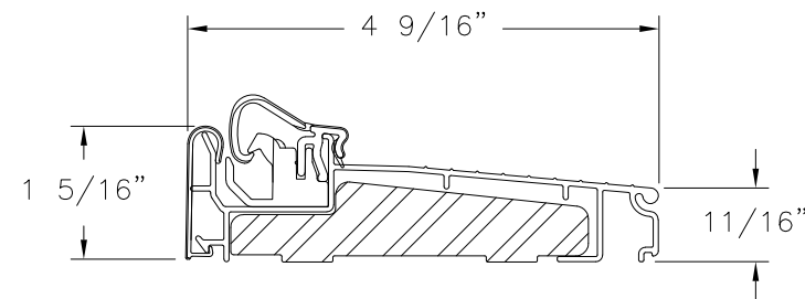
INSWING SILL ZAQL4565
