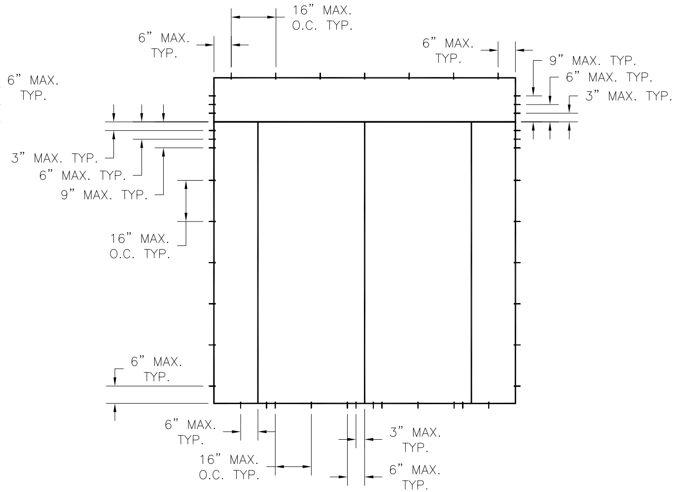
DOUBLE W/SIDELITES & TRANSOM
