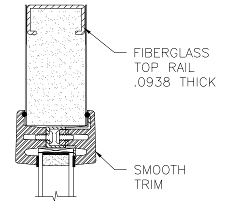
OPTION 21 SMOOTH TRIM W/TAPE
