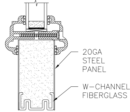
OPTION 25 ELTON TRIM
