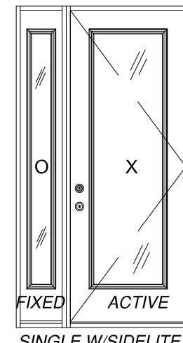
SINGLE W/SIDELITE
