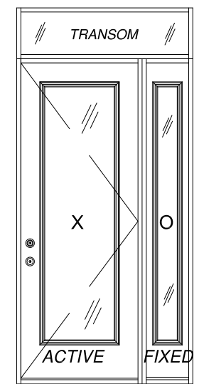
SINGLE W/SIDELITE & TRANSOM
