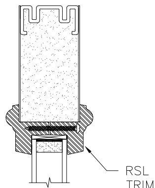
OPTION 15 SMOOTH TRIM
