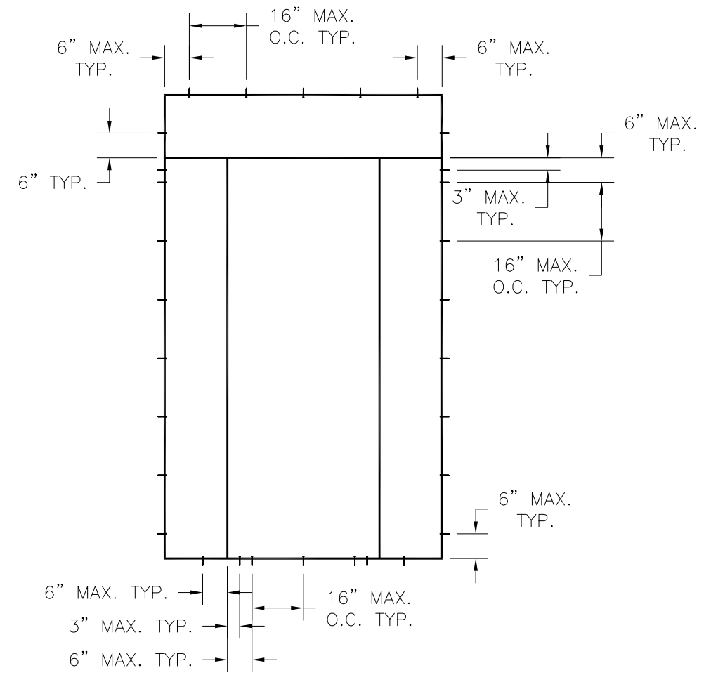
SINGLE W/SIDELITES & TRANSOM
