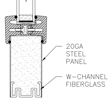
OPTION 15 SMOOTH TRIM
