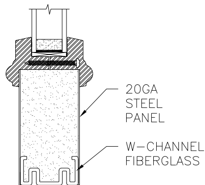
OPTION 18 RSL TRIM
