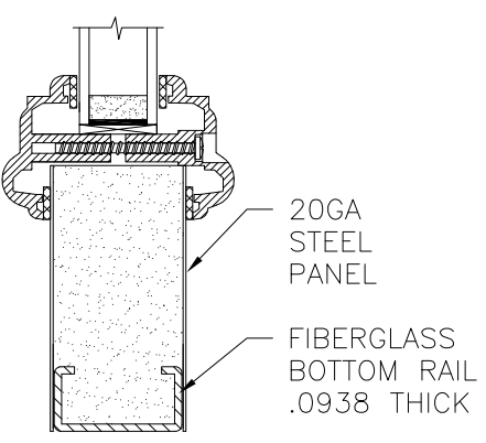
OPTION 20 ELTON TRIM
