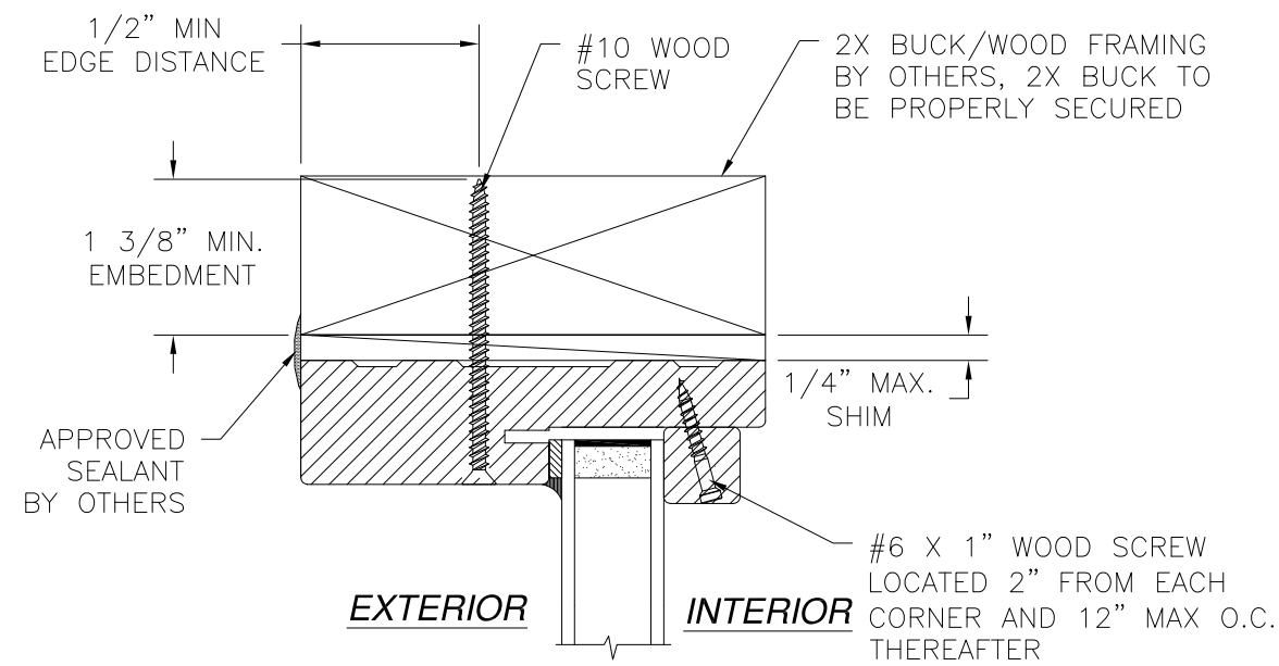
TRANSOM DETAIL INSWING/OUTSWING 2X BUCK/WOOD FRAMING INSTALLATION HEAD SHOWN JAMBS SIMILAR
