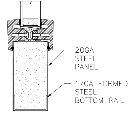
OPTION 24 SMOOTH TRIM W/TAPE
