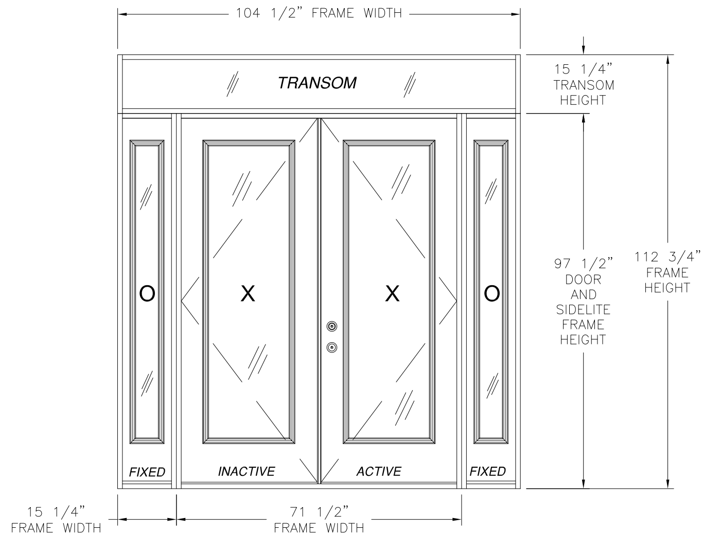
20GA STEEL OS DOUBLE DOOR W/ SIDELITES AND TRANSOM EXTERIOR VIEW
