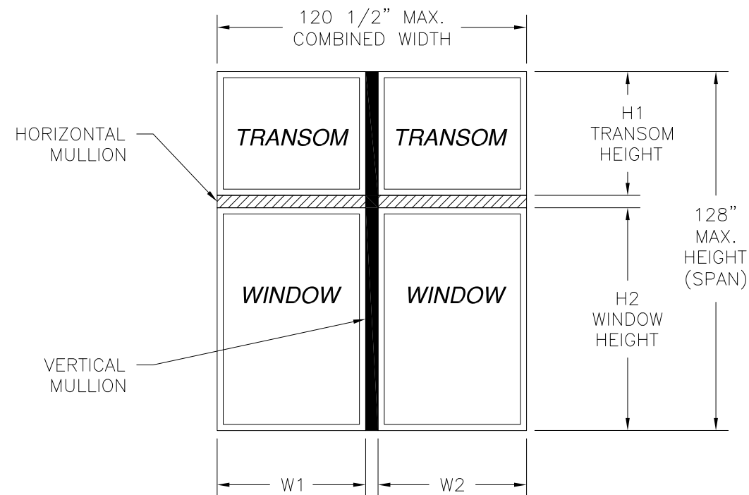
10300085 ALUMINUM X MULLION NON REINFORCED IMPACT UP TO WIND ZONE 3
