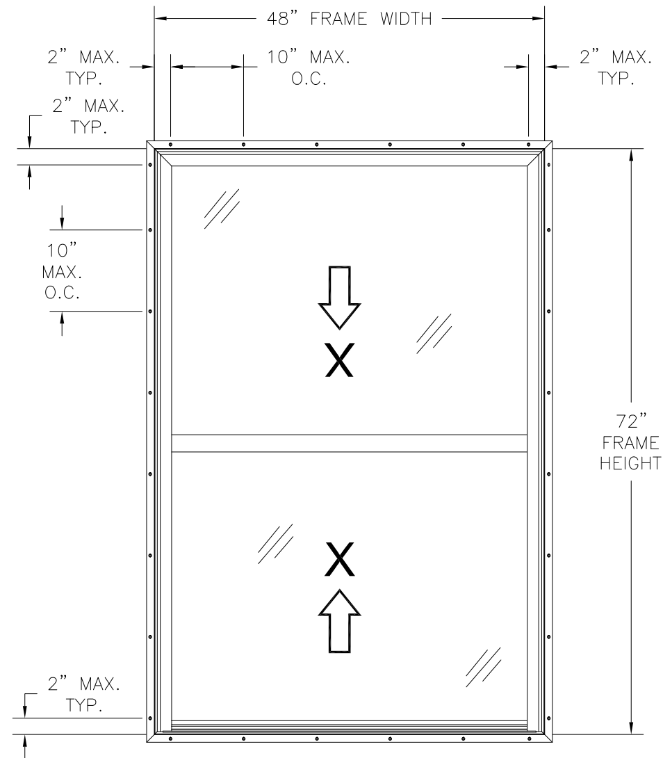
STORMGATE NC DH PVC DOUBLE HUNG WINDOW EXTERIOR VIEW
