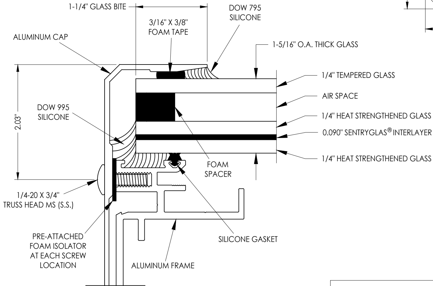
G1 GLAZING DETAIL MISSILE LEVEL "D"
