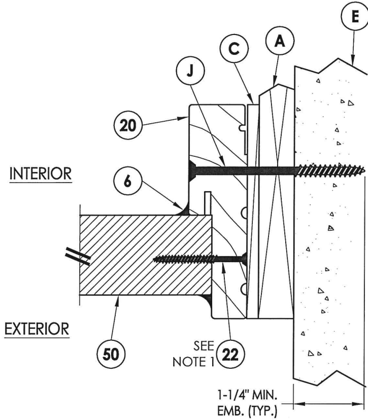
4 4 HORIZONTAL CROSS SECTION Shown w/1X sub-buck
