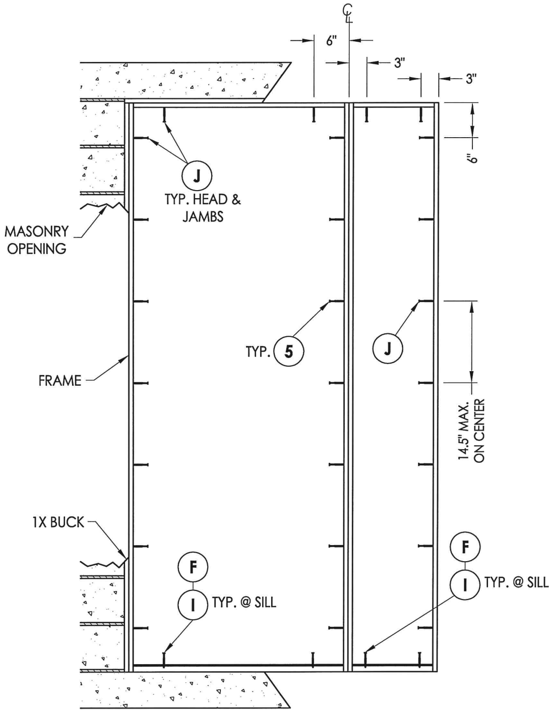
FRAME ANCHORING Masonry 1X buck construction
