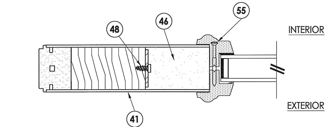
1 2 HORIZONTAL CROSS SECTION
