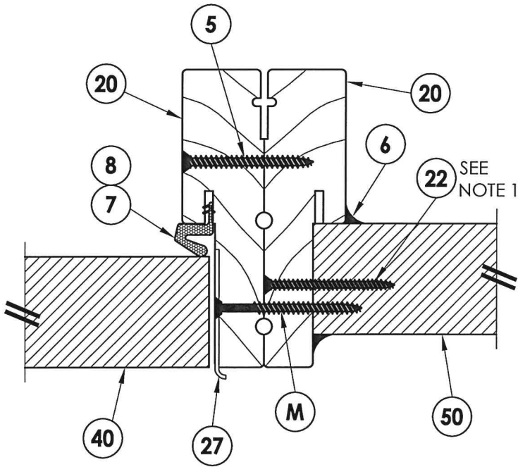
2 4 HORIZONTAL CROSS SECTION Outswing shown - inswing also approved
