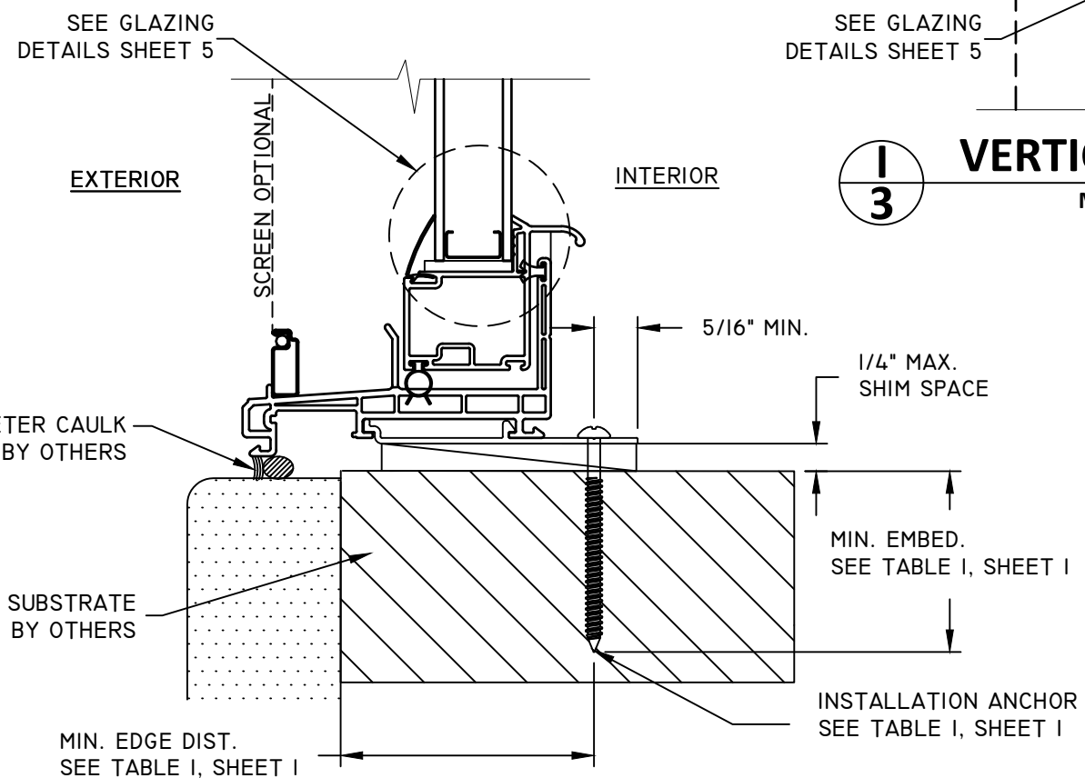
A 3 VERTICAL SECTION SILL BRICKMOULD FRAME - CLIP INSTALLATION
