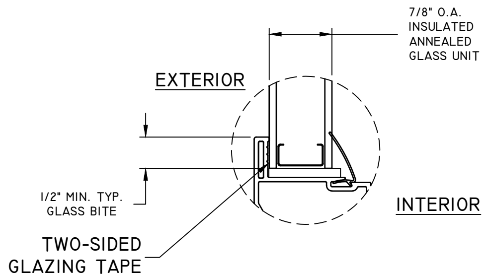
GLAZING DETAIL 2
