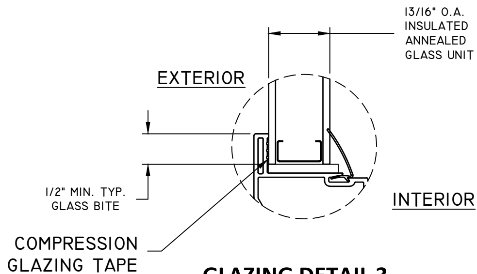
GLAZING DETAIL 3
