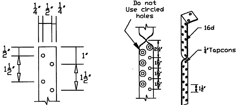
NVRT Anchor Holes dia. \frac{3}{16} "
