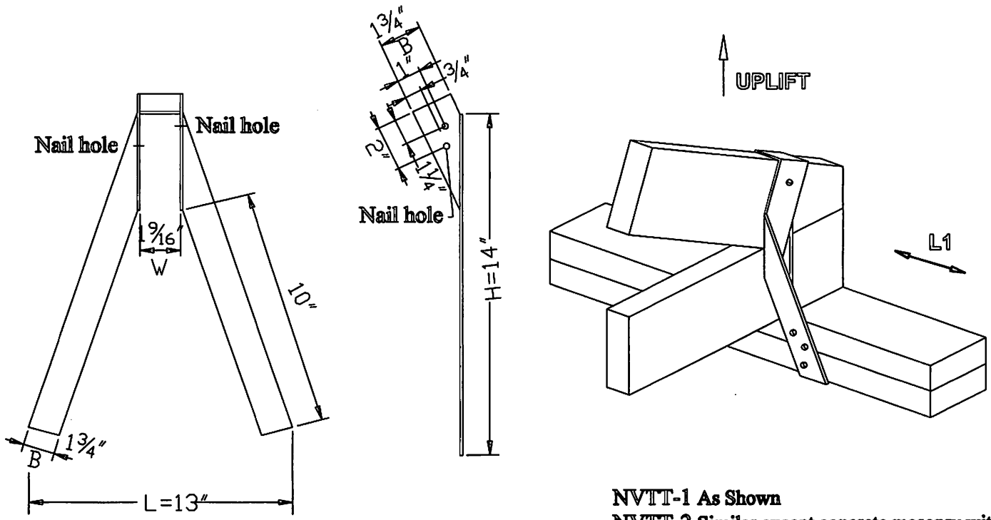
NVTT 1 and 2
