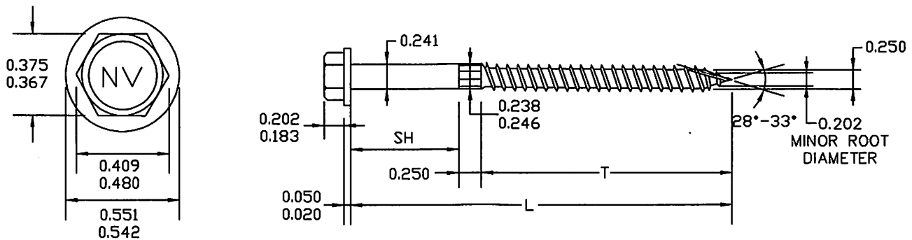
NVWS SCREW
