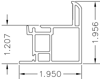
⑤ SL77S LOCK STILE 0.079" EXT. WALL THK. 0.059 INT. WALL THK.
