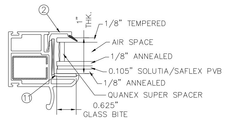
GLAZING DETAIL WITH SOLUTIA/SAFLEX LAMINATE
