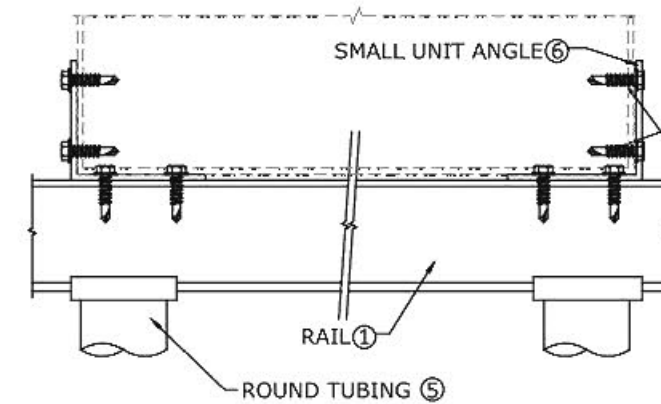
SECTION C-C (SIDE-VIEW)
