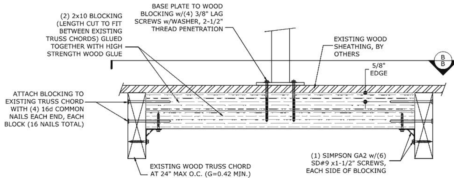
SECTION A-A (SECTION-VIEW)
