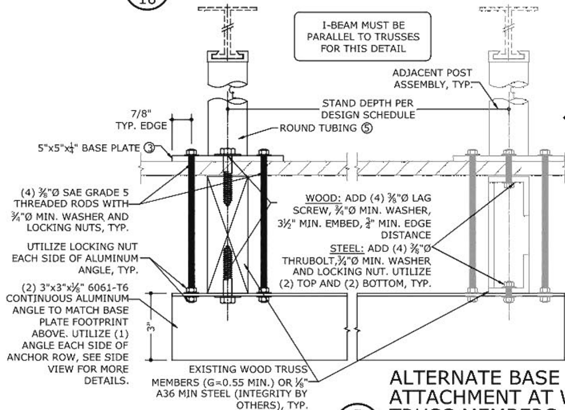
5 16 ALTERNATE BASE PLATE ATTACHMENT AT WOOD/STEEL TRUSS MEMBERS
