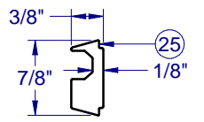
REINF. EXTERNAL S-2011
