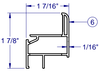
PVC SASH FMR H-6137
