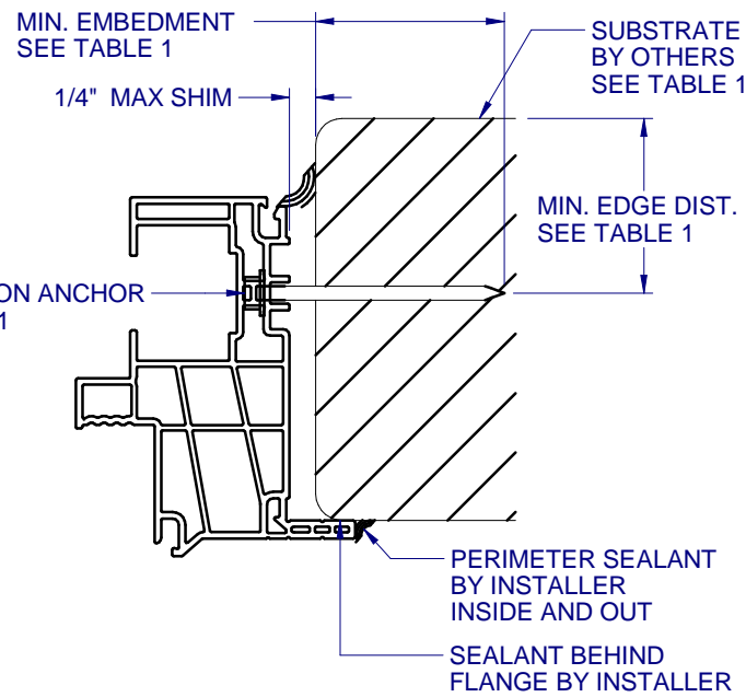
B HORIZONTAL SECTION 7 TYPICAL JAMB ANCHORAGE
