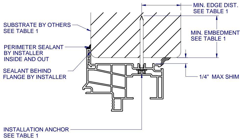
TYPICAL HEAD ANCHORAGE
