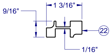
REINF. BTM RAIL S-2007
