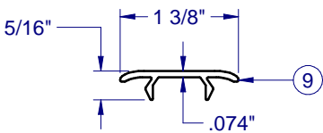
PVC SASH STOP S-6138
