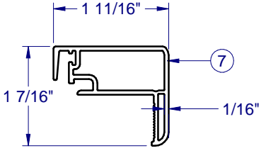
PVC SASH TOP RAIL H-6138
