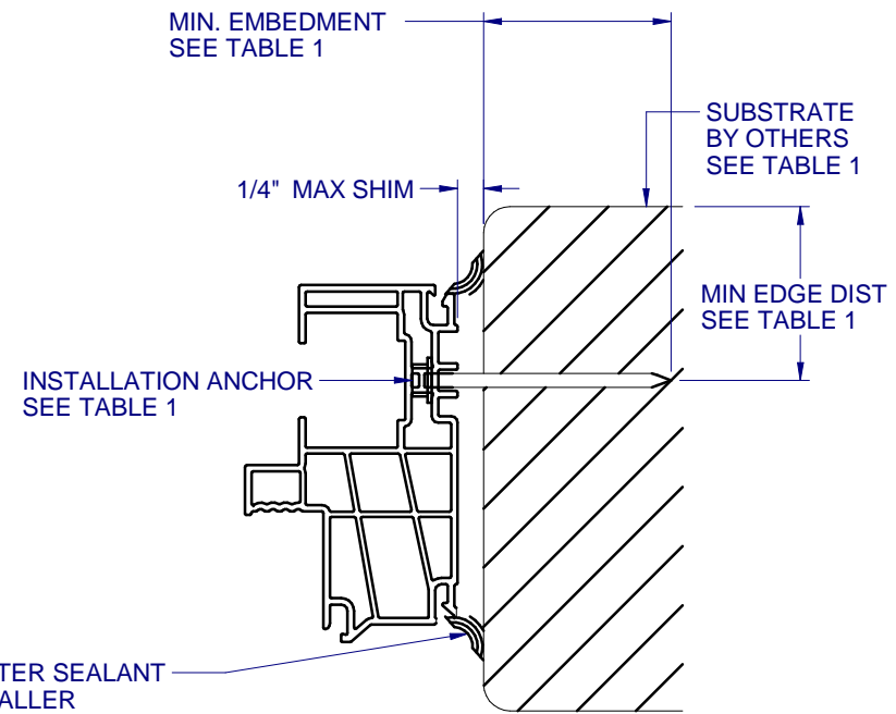
D HORIZONTAL SECTION 7 BOX FRAME INSTALLATION SIMILAR FOR SILL AND JAMBS FOR BOX INSTALLATION
