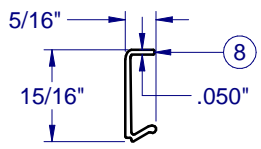
PVC GLAZING BEAD S-6141
