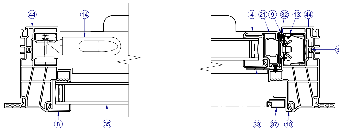
SECTION B-B
