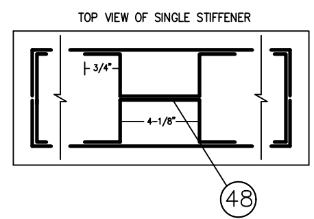
22GA. STIFFENER DETAIL PANIC DEVICE
