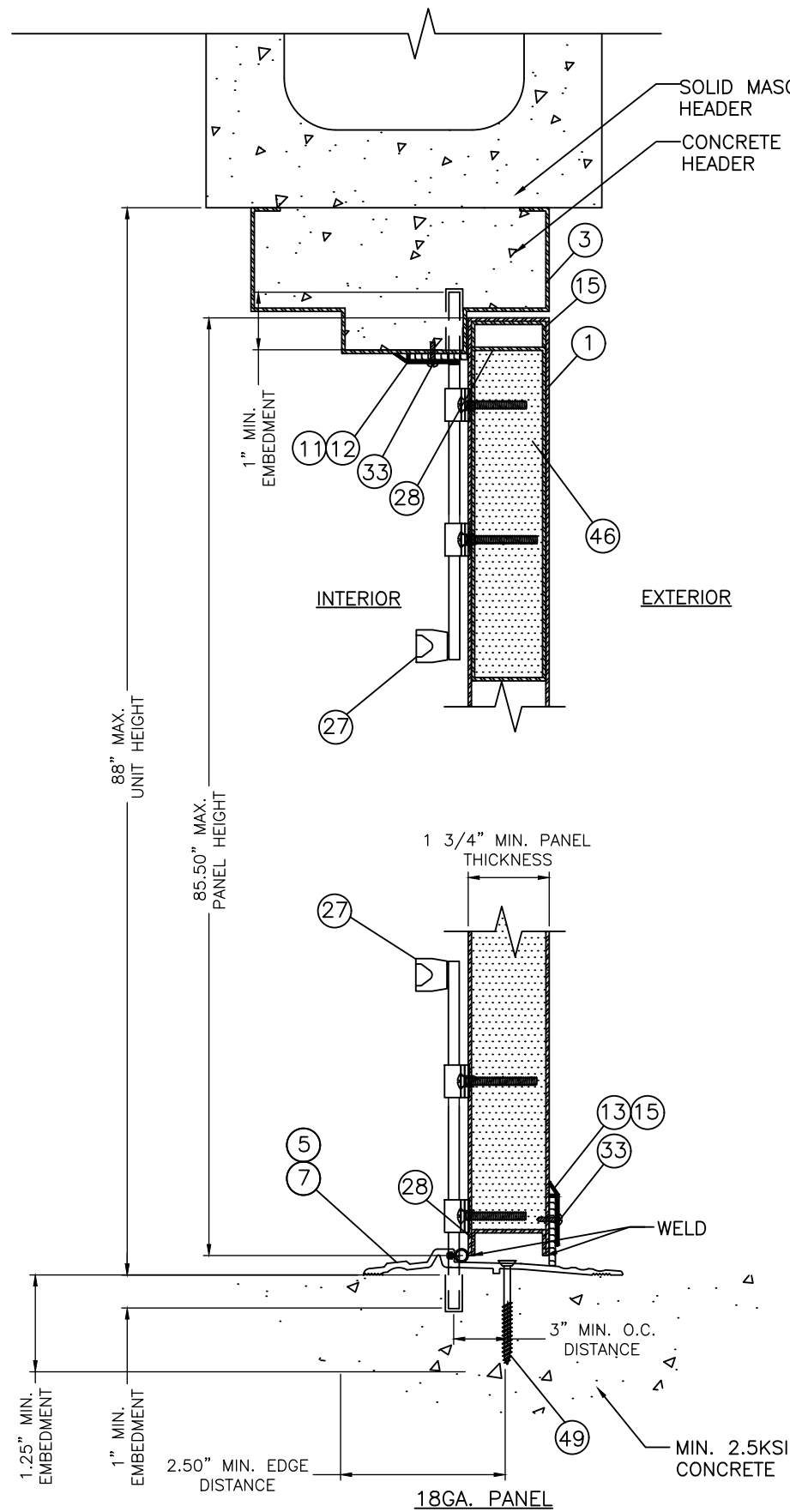
A VERTICAL SECTION 7 HEAD/SILL - CONCRETE / GROUT - FILLED CMU (MORTISE LOCK/ CYLINDRICAL LOCK WITH SURFACE BOLTS)
