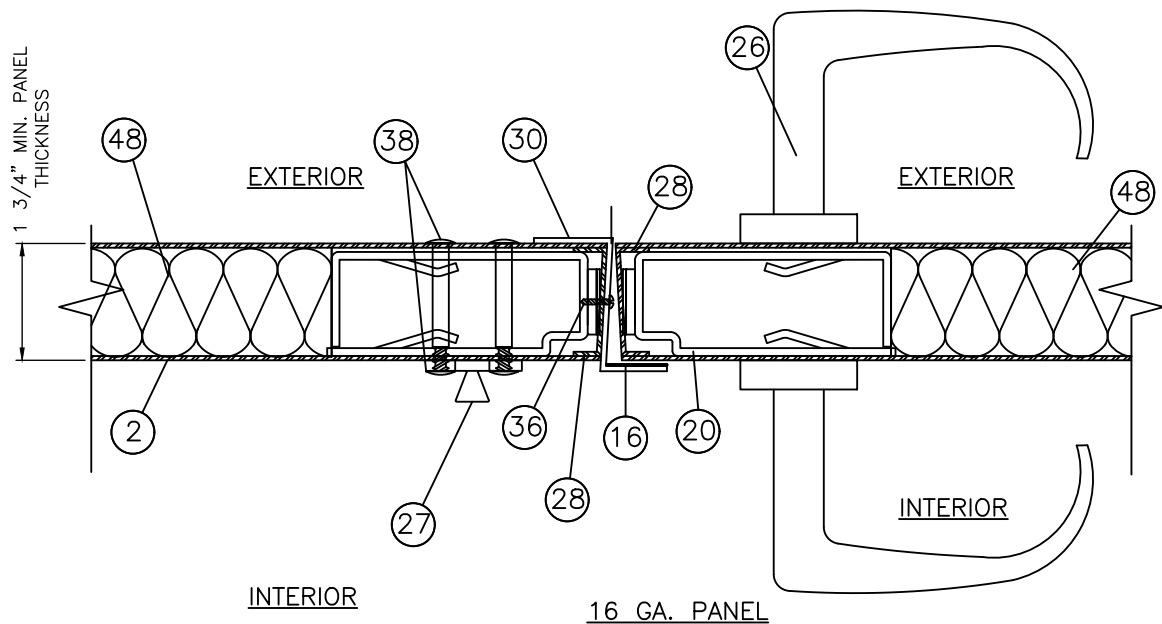
L 10 HORIZONTAL SECTION CORBIN/RUSSWIN ML2000 MORTISE LOCKSET
