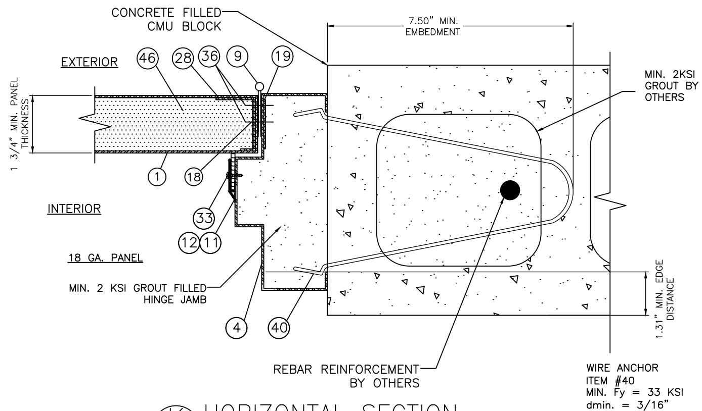
K 9 HORIZONTAL SECTION JAMB - CONCRETE/MASONRY WIRE ACNCHOR/HMF 18GA PANEL
