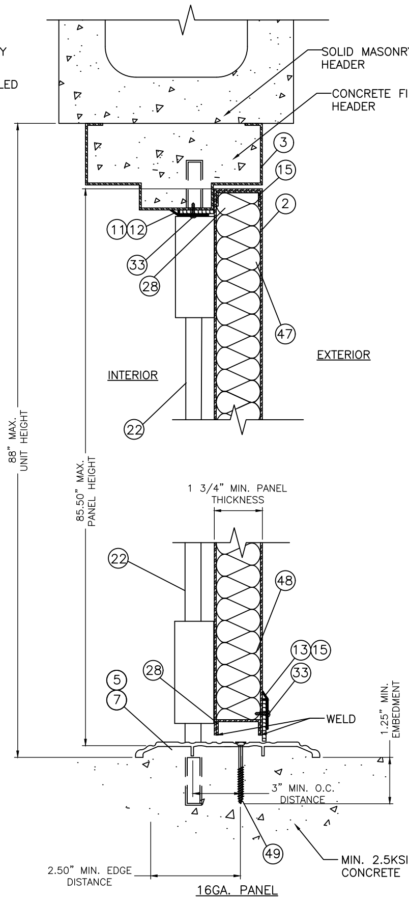
B VERTICAL SECTION 7 HEAD/SILL - CONCRETE / GROUT - FILLED CMU (SURFACE VERTICAL ROD)
