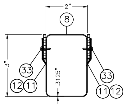
MULLION DETAIL C DORMA HC1300 REMOVABLE MULLION (SEE MULLION TOP & BOTTOM INSTALLATION DETAILS, SHEET 6)
