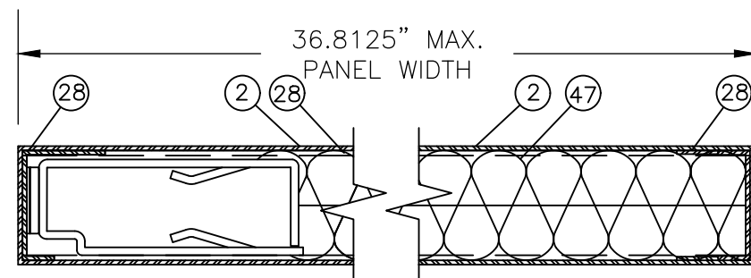
HMF 16 GA. PANEL HORIZONTAL CROSS SECTION (FOR ILLUSTRATION ONLY)
