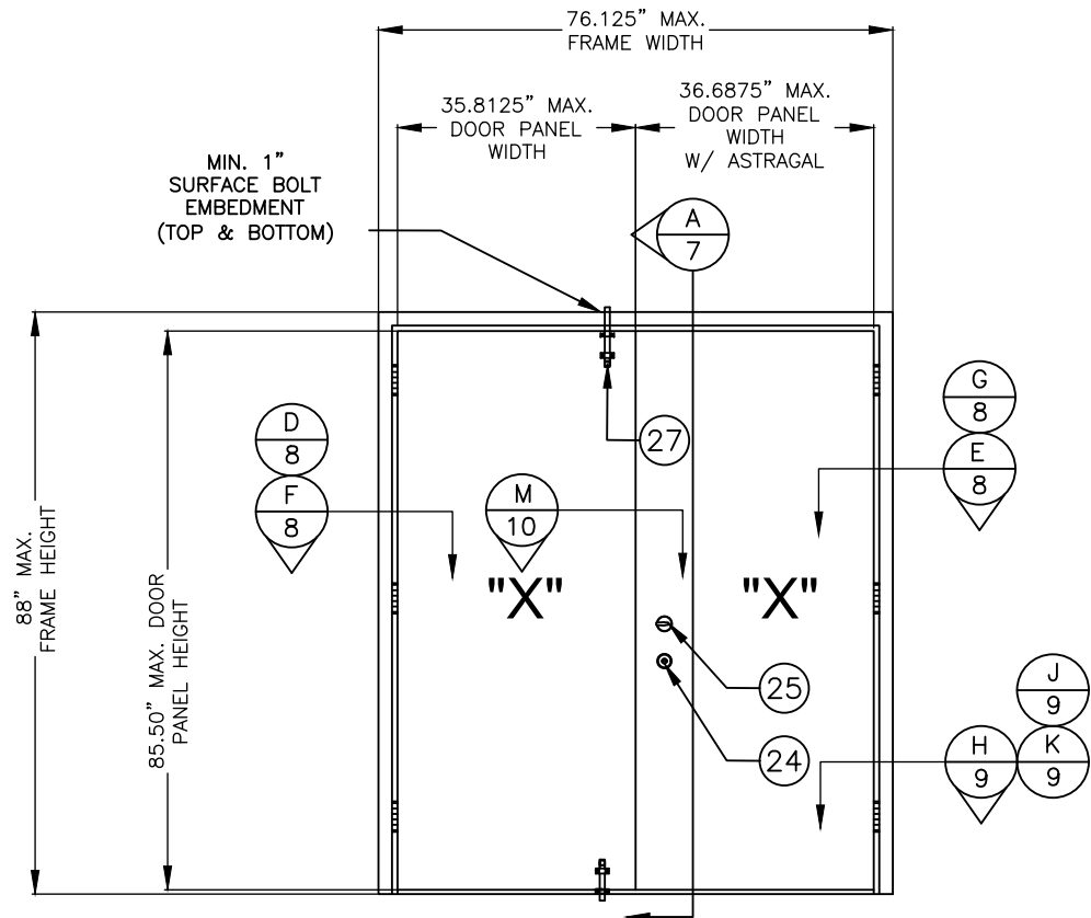
ELEVATION INTERIOR VIEW CORBIN/RUSSWIN 26D HEAVY DUTY CYLINDRICAL LOCKSET DL3000 CYLINDRICAL DEAD LOCK
