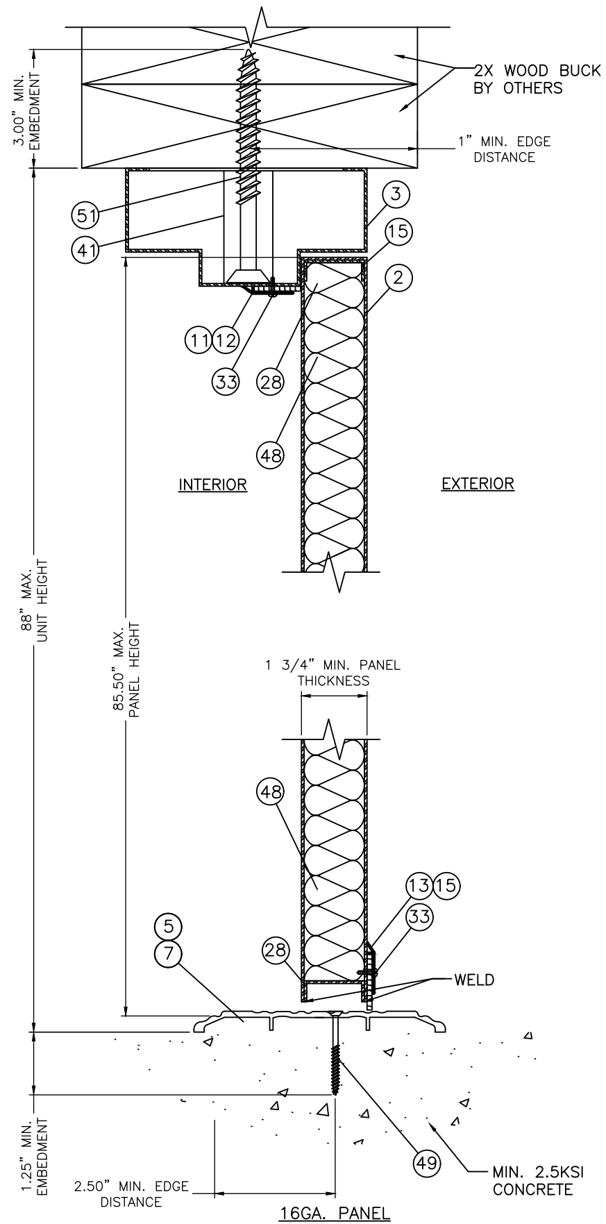
C VERTICAL SECTION 7 HEAD - 2X WOOD FRAME SILL - CONCRETE (REMOVABLE MULLION)
