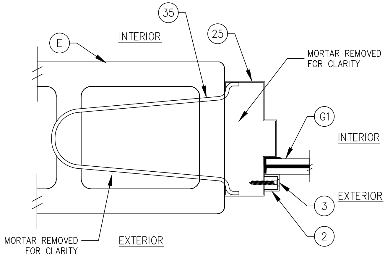
1 HORIZONTAL CROSS SECTION 3 NEW MASONRY
