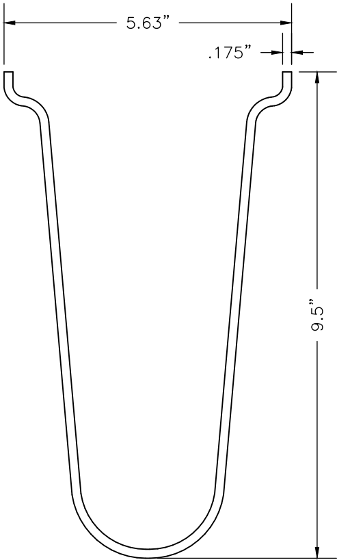
35 WIRE ANCHOR
