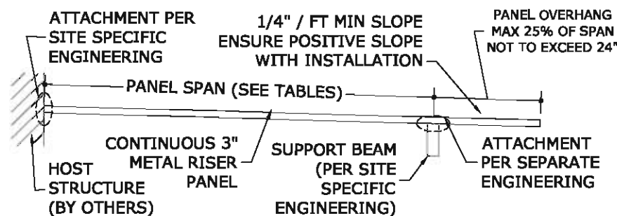
3 3" METAL RISER ROOF PANELS 1 N.T.S. ELEVATION
