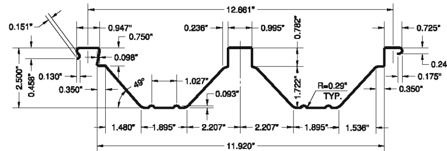
1 3" METAL RISER PANELS 1 N.T.S. SECTION VIEW
