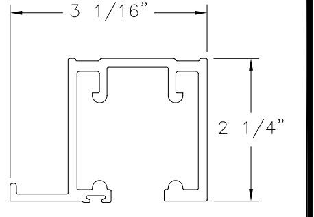
HEAD TRACK ALUMINUM 6063-T5
