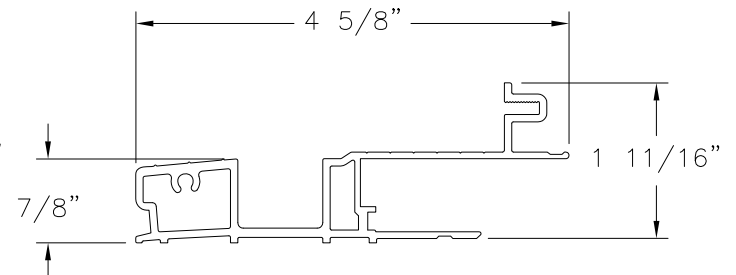
OUTSWING SILL-B ALUMINUM 6063-T5
