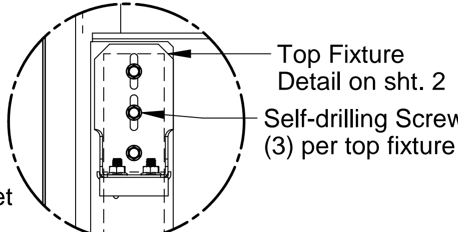
Top Fixture Attachment
