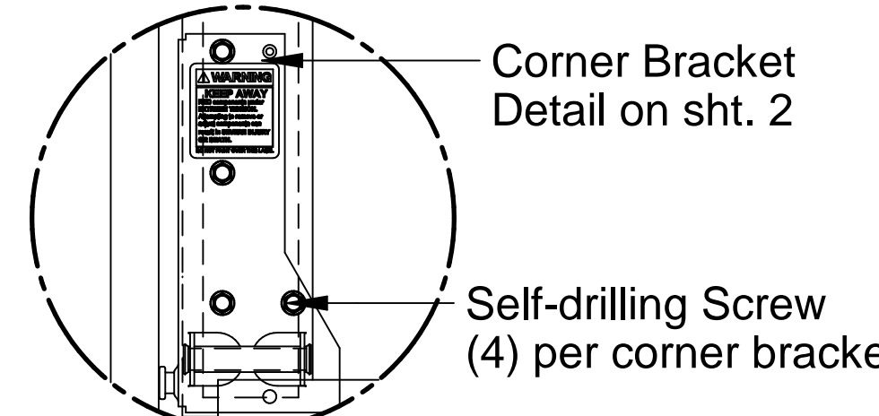
Corner Bracket Attachment
