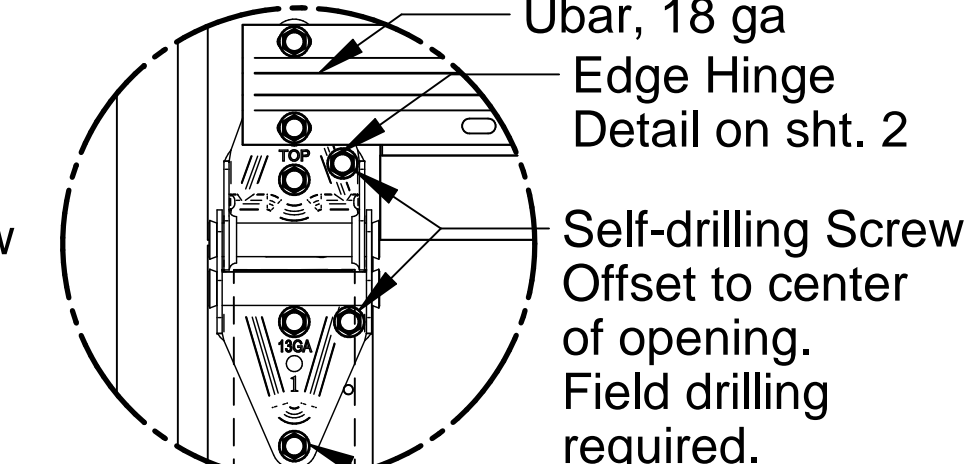
Edge Hinge Attachment
