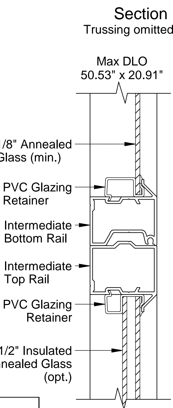
Section C-C
