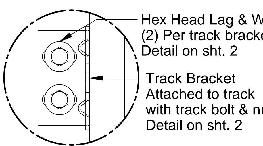
Track Bracket Attachment Alternate mounting details on sht. 4
