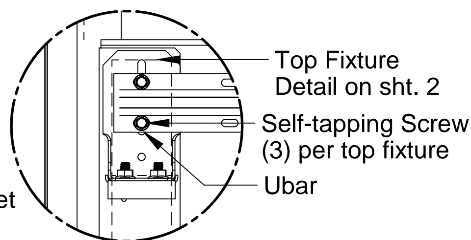
Top Fixture Attachment
