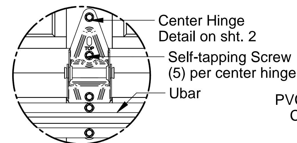
Center Hinge Attachment
