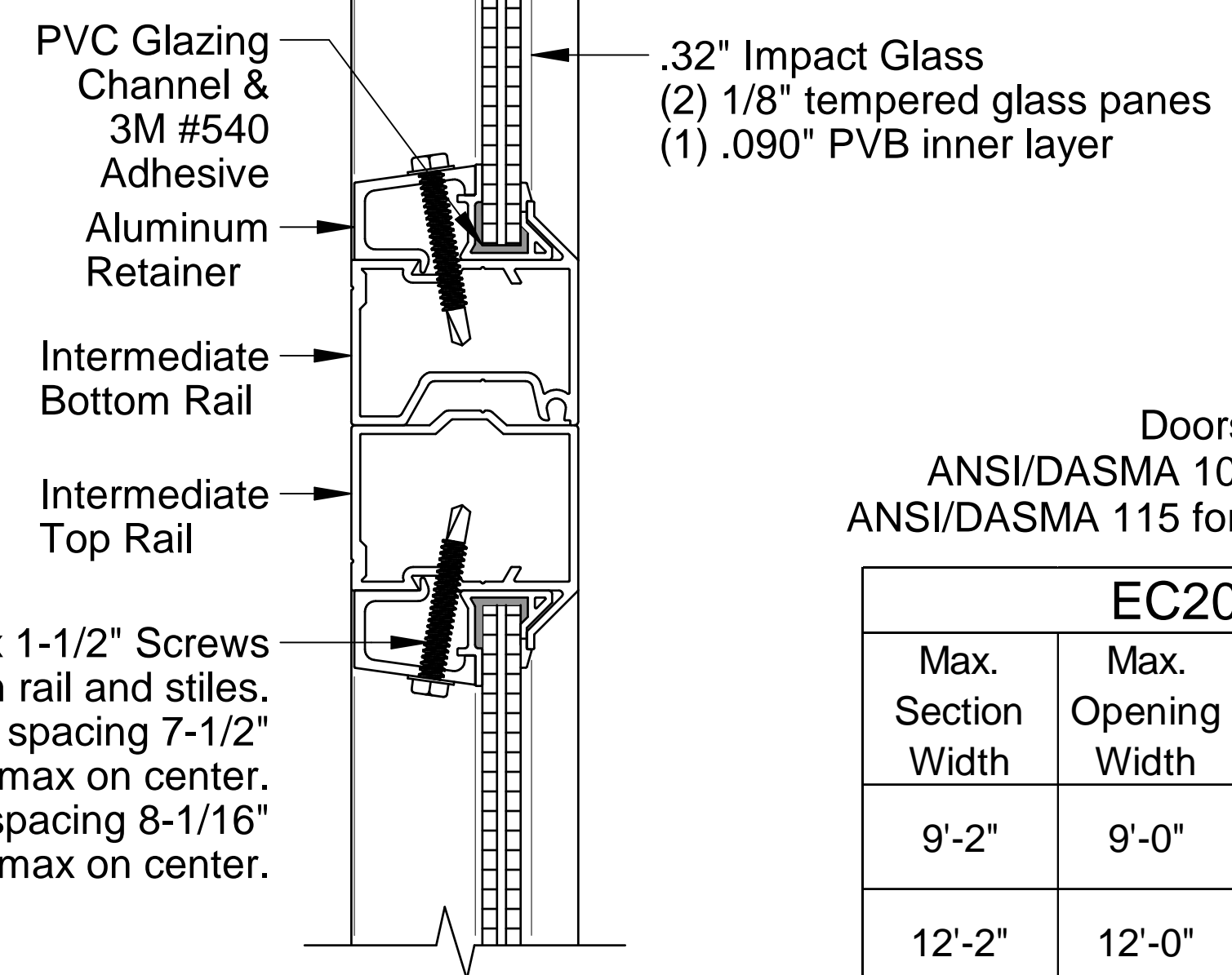
Section C-C
