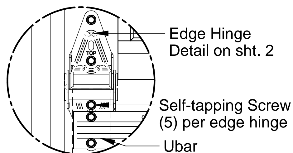
Edge Hinge Attachment
