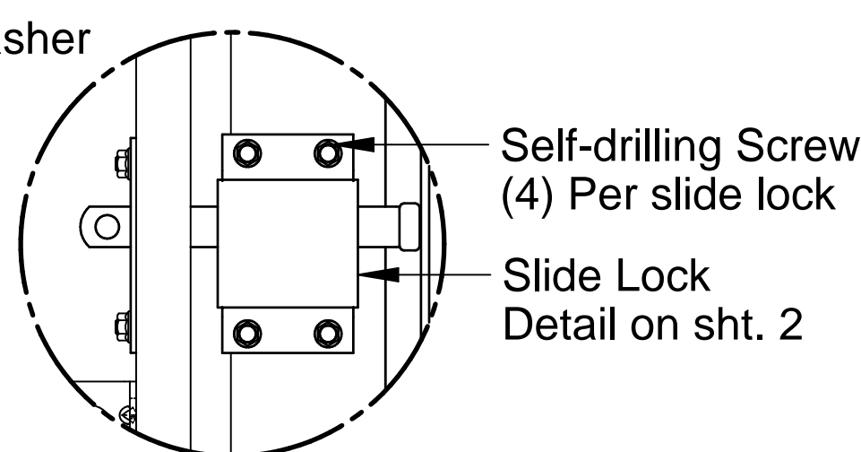
Slide Lock Attachment Required on doors without operators.
