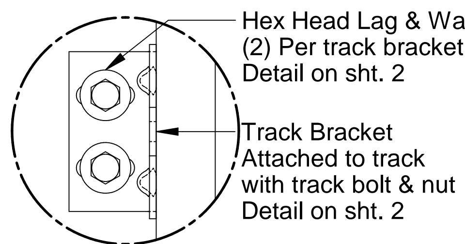
Track Bracket Attachment Alternate mounting details on sht. 4
