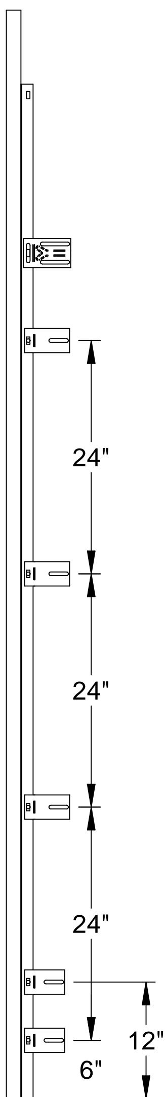
Clip Angle to Structure: Track Leg Spacing
