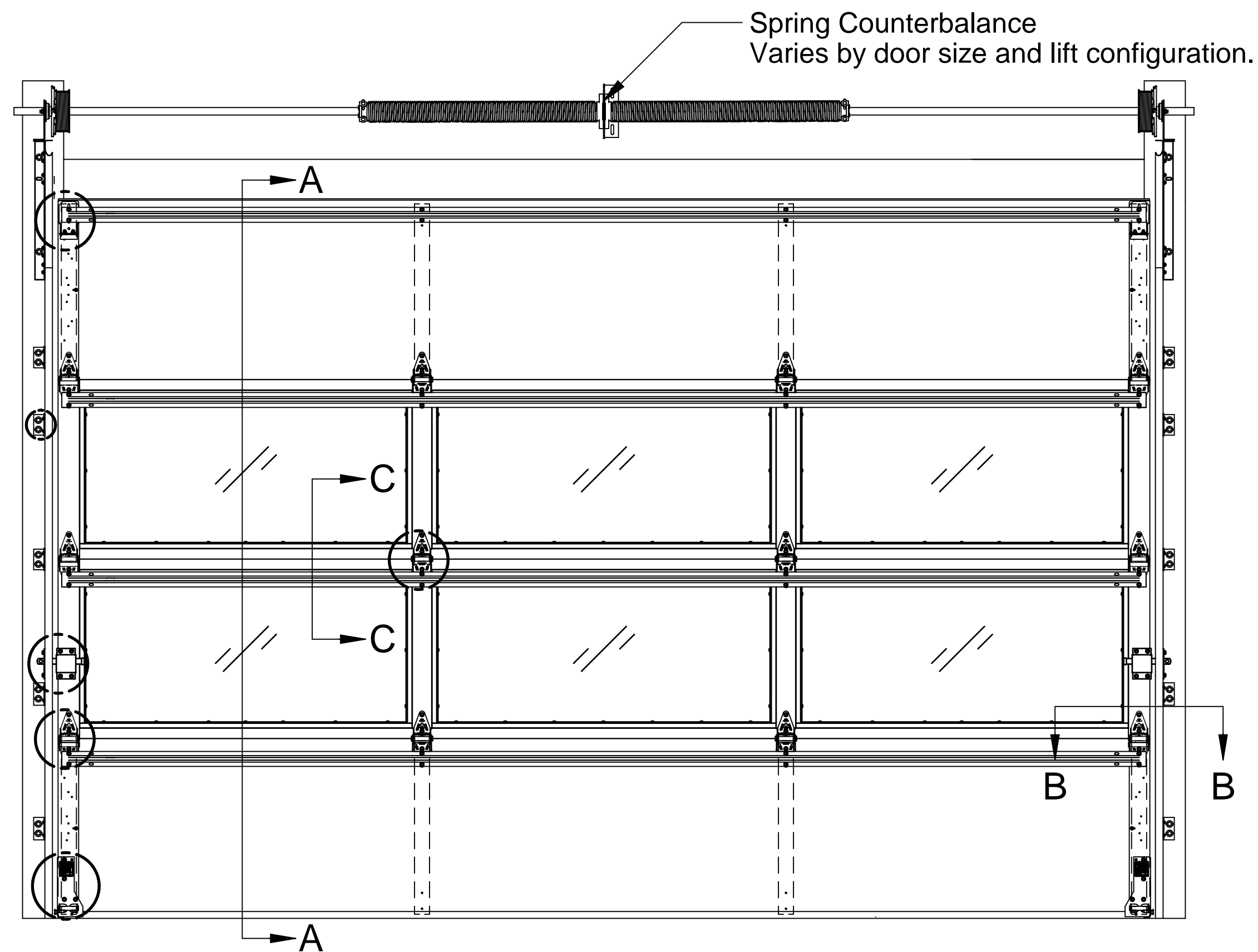
Interior Elevation
