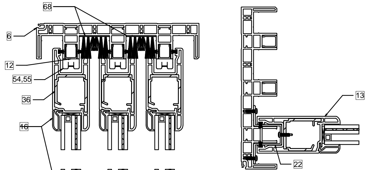
FIXED PANEL ATTACHMENT
