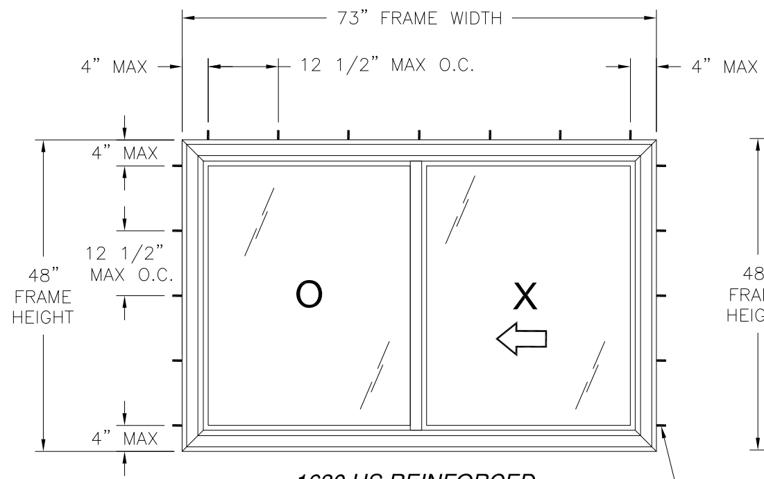
1630 HS REINFORCED EXTERIOR VIEW FINLESS & FLANGE INSTALLATION
