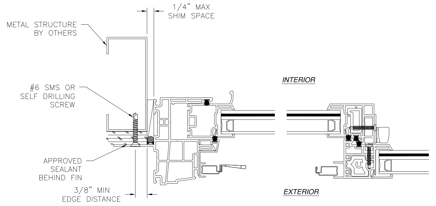
JAMB INSTALLATION DETAIL METAL STRUCTURE INSTALLATION
