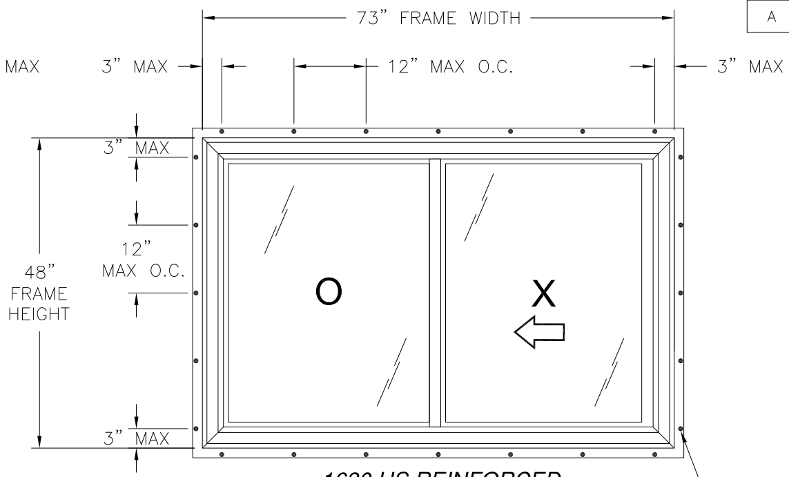
1630 HS REINFORCED EXTERIOR VIEW FIN INSTALLATION
