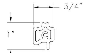
MEETING RAIL REINFORCEMENT (M-2343) ALUMINUM 6063-T5
