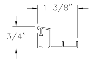
OPERABLE SCREEN TRACK (M-2340) ALUMINUM 6063-T5
