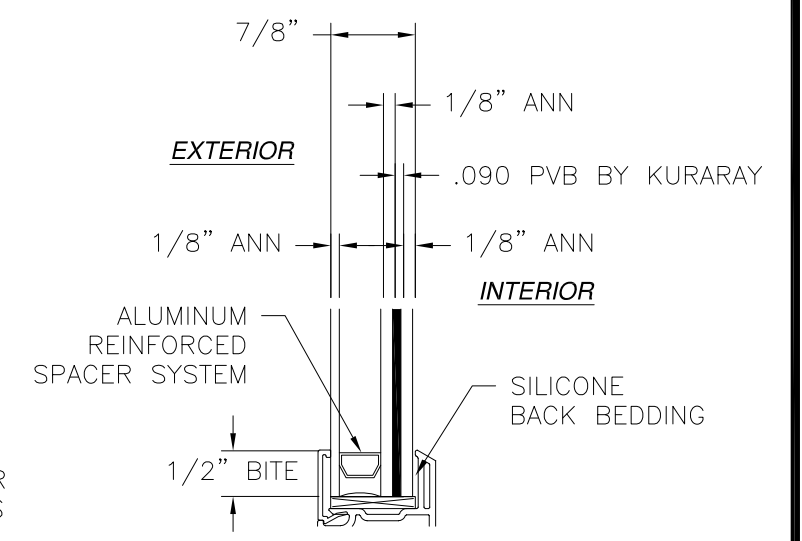
GLAZING DETAIL
