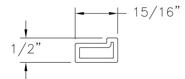
LOCK RAIL REINFORCEMENT (M-2115) ALUMINUM 6063-T5
