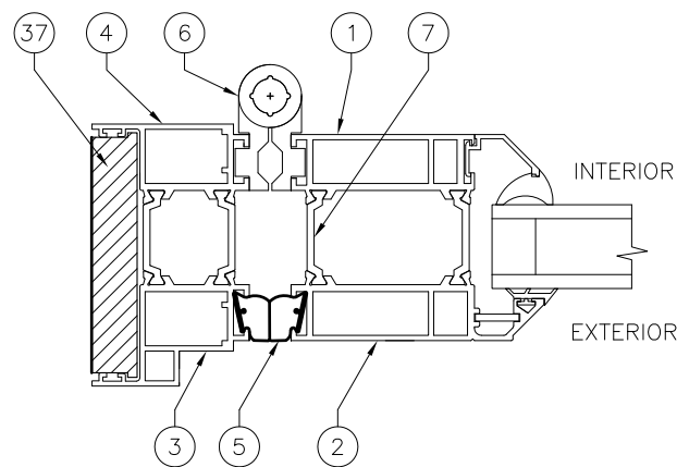
DETAIL H1. OPEN-IN HINGE JAMB, REVERSE HINGES (6) AND JAMB (3&4) FOR OPEN-OUT
