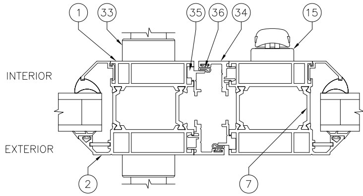
DETAIL H3. OPEN-OUT LOCKING MEETING STILES, REVERSE PARTS 34 AND 35 FOR OPEN-IN
