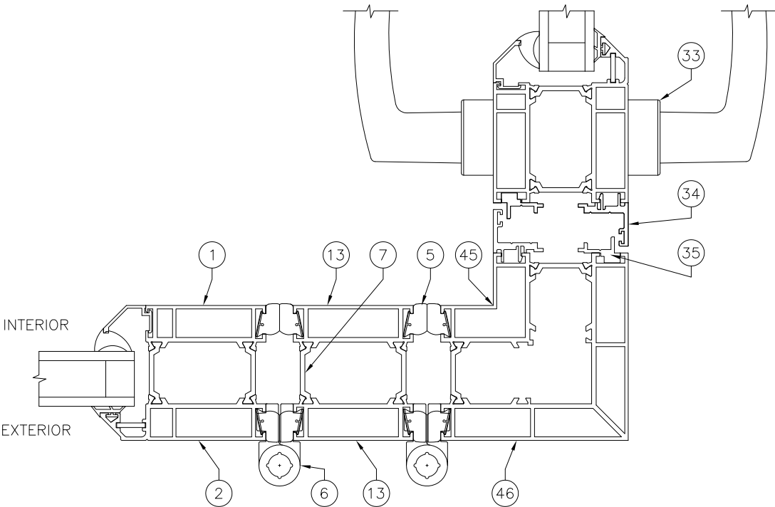
DETAIL H5. OPEN-OUT OUTSIDE 90-DEG. CORNER MULLION
