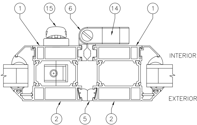
DETAIL H2. OPEN-OUT STILES, REVERSE HINGES FOR OPEN-IN
