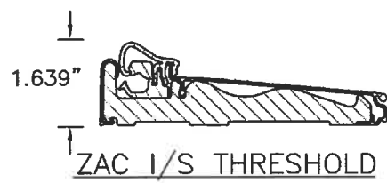
DETAIL "C"
