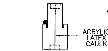
COMBINATION WOOD MULLION (BOXED)
