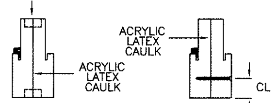
COMBINATION WOOD MULLION (BOXED)
