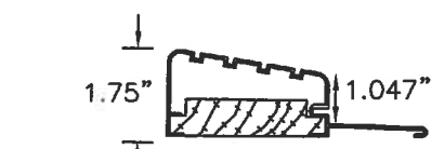
HIGH DAM O/S THRESHOLD
