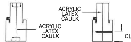
COMBINATION WOOD MULLION (BOXED) COMBINATION WOOD MULLION (BOXED)
