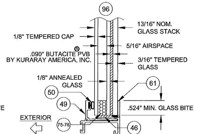
13/16" I.G. GLAZING DETAIL
