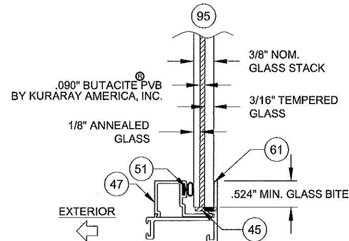
3/8" GLAZING DETAIL
