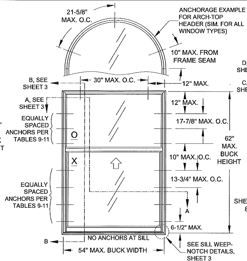
ELEVATION FOR TYP. FLANGE FRAME SHOWN WITH STANDARD COTTAGE CONFIGURATION FOR CUSTOM COTTAGE CONFIGURATION UP TO 75" HEIGHT SEE TABLES 7-11
