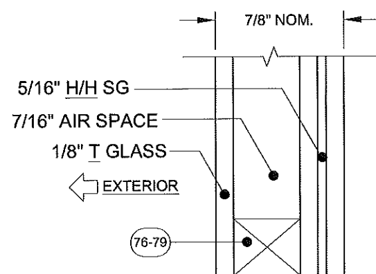
GLASS TYPE 10
