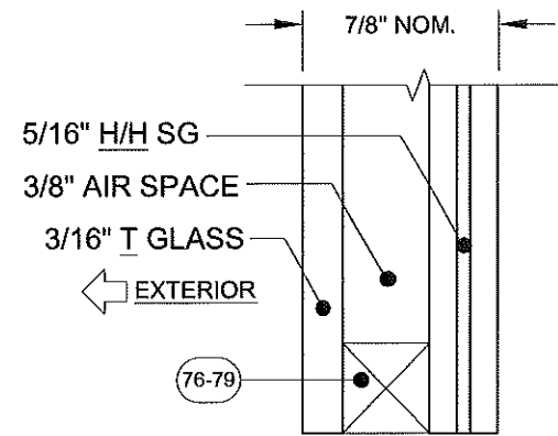
GLASS TYPE 12
