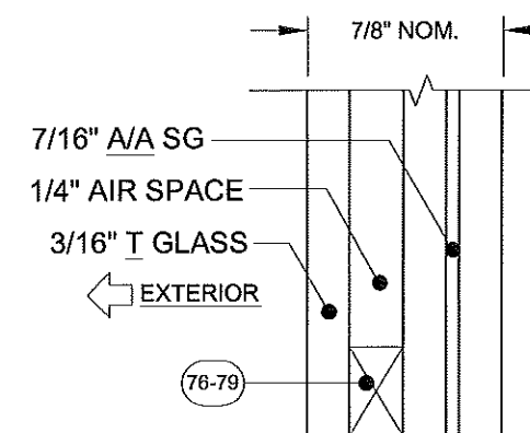
GLASS TYPE 16
