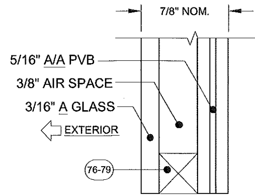
GLASS TYPE 7
