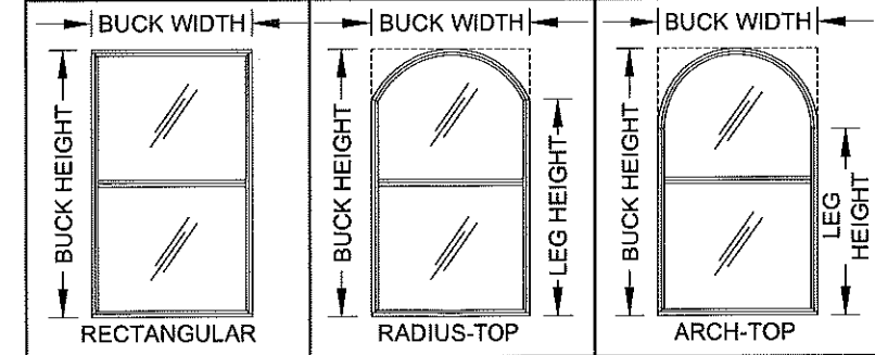
FIGURE C: FRAME SHAPES
