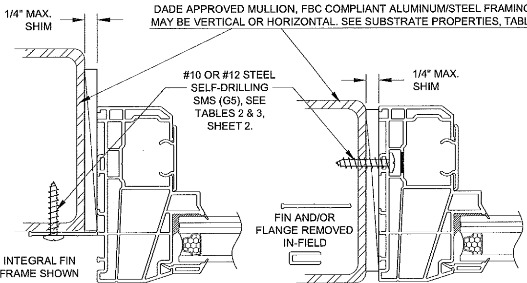
HORIZONTAL SECTION C-C
