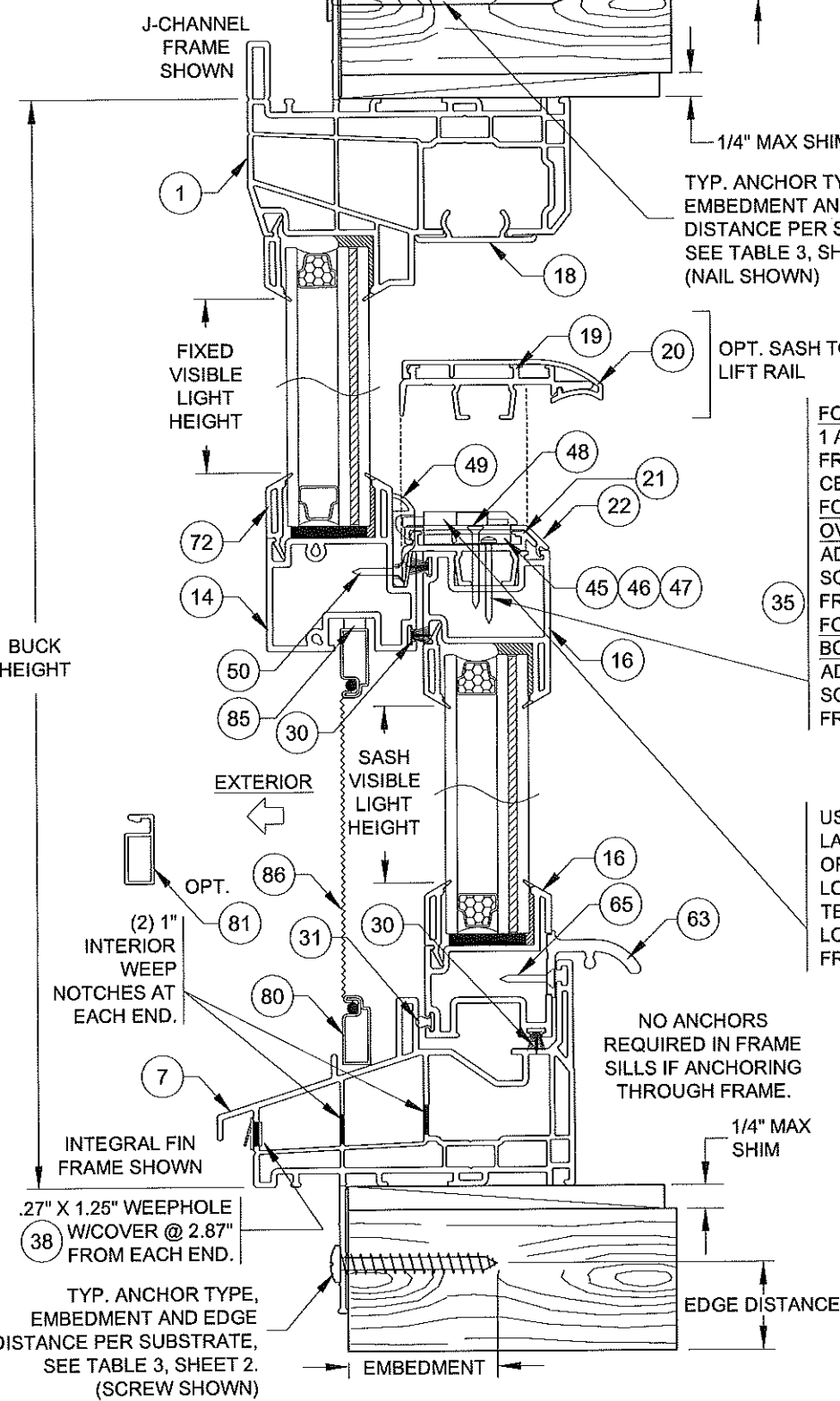
VERTICAL SECTION D-D
