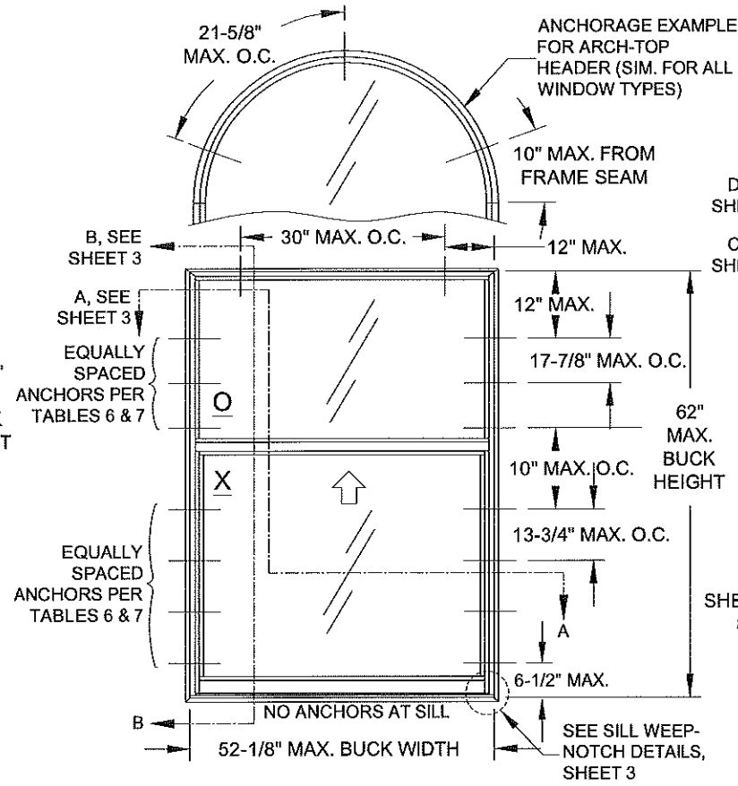
ELEVATION FOR TYP. FLANGE FRAME SHOWN WITH STANDARD COTTAGE CONFIGURATION FOR CUSTOM COTTAGE CONFIGURATION UP TO 75" HEIGHT SEE TABLES 6 & 7
