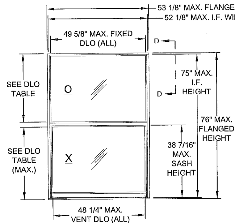
DETAIL A 1/1
