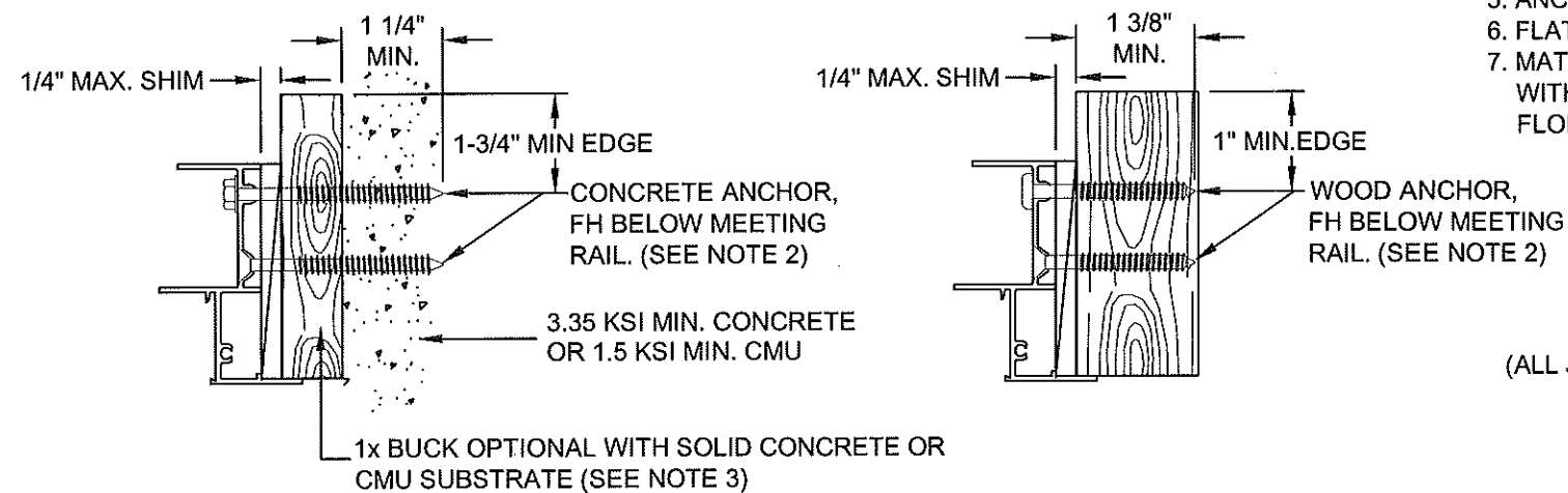
TYPICAL FLANGED JAMB ANCHORAGE
