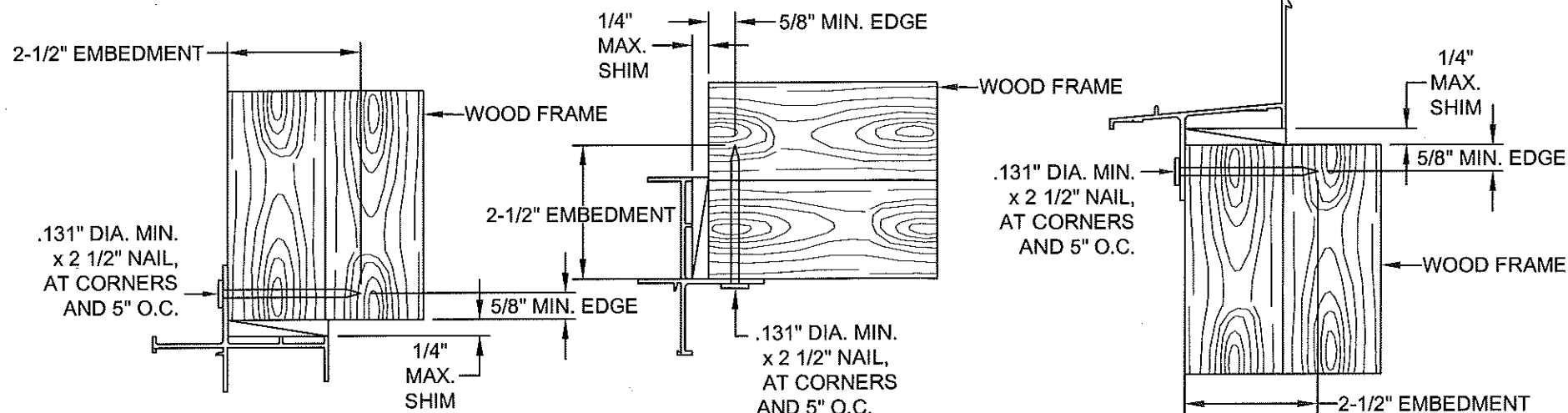
TYPICAL FLANGED JAMB ANCHORAGE
