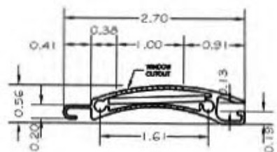
A1 - 58 mm VIEW PORT SLATS (VENTED OR SOLID) 6063-T6 EXTRUDED ALUMINUM
