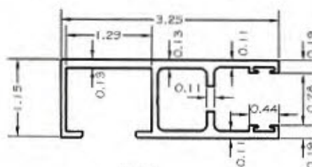
C1 - ROLLING WALL GUIDE RAIL WITH SNAP COVER 6063-T6 EXTRUDED ALUMINUM
