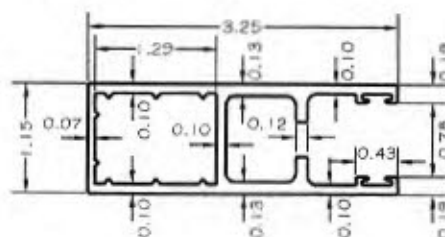
C- ROLLING WALL GUIDE RAIL 6063-T6 EXTRUDED ALUMINUM
