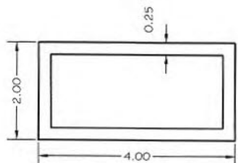
F-TUBE EXTRUDED ALUMINUM 6061-T6 or 6005-T5
