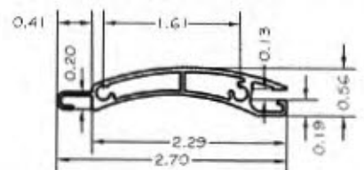
A1 - 58 mm VIEW PORT SLATS (VENTED OR SOLID) 6063-T6 EXTRUDED ALUMINUM
