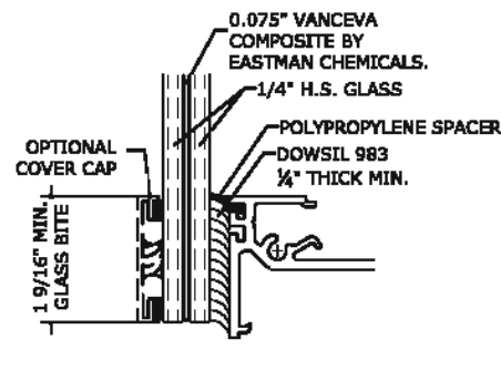
GLASS TYPE J GLAZING DETAIL N.T.S. GLASS RATING: LARGE MISSILE LEVEL D 3/16" GLASS
