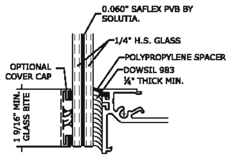
GLASS TYPE H GLAZING DETAIL N.T.S. GLASS RATING: LARGE MISSILE LEVEL D 3/16" GLASS
