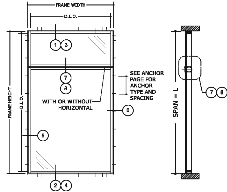
TYPICAL SINGLE PANEL OPENING
