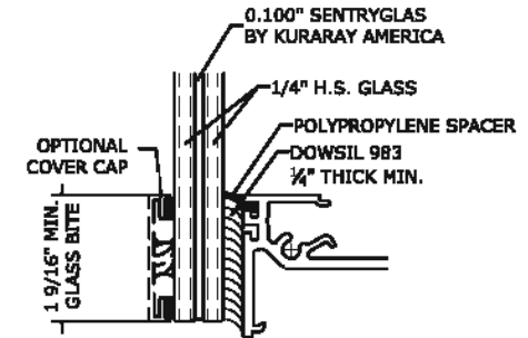
GLASS TYPE A GLAZING DETAIL N.T.S. GLASS RATING: LARGE MISSILE LEVEL D 3/8" GLASS
