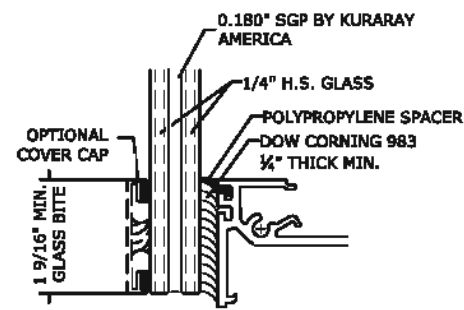
GLASS TYPE K GLAZING DETAIL N.T.S. GLASS RATING: LARGE MISSILE LEVEL E 3/8" GLASS
