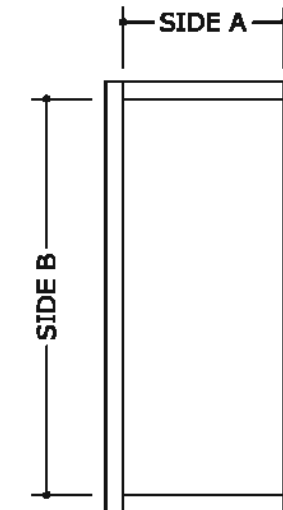
GLASS TYPE D1 GLAZING DETAIL N.T.S. GLASS RATING: LARGE MISSILE LEVEL D 1 3/8" GLASS
