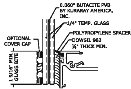
GLASS TYPE G GLAZING DETAIL
