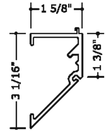
24 270° CORNER ADAPTOR
