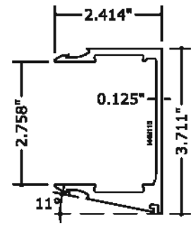
8A MALE JAMB / MULLION
