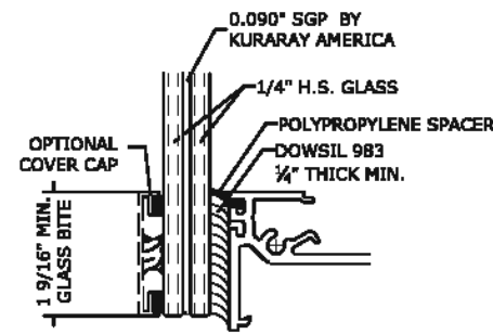
GLASS TYPE I GLAZING DETAIL
