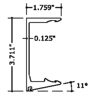
7A FEMALE JAMB / MULLION
