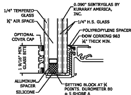
GLASS TYPE B1 GLAZING DETAIL N.T.S. GLASS RATING: LARGE MISSILE LEVEL D 1 1/8" GLASS
