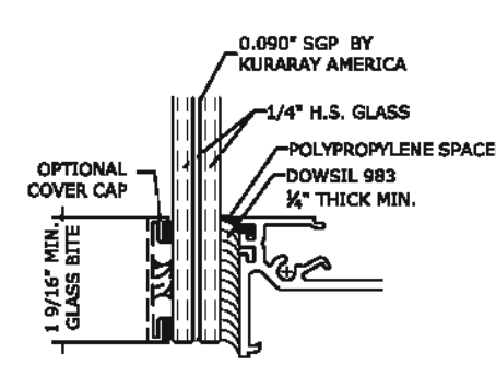
GLASS TYPE I GLAZING DETAIL N.T.S. GLASS RATING: LARGE MISSILE LEVEL D 3/16" GLASS
