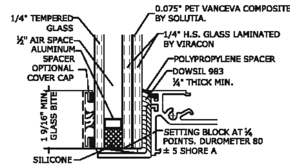
GLASS TYPE C1 GLAZING DETAIL N.T.S. GLASS RATING: LARGE MISSILE LEVEL E 1 3/8" GLASS
