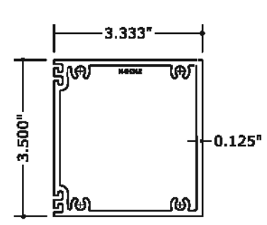
6 HORIZONTAL INTERMEDIATE
