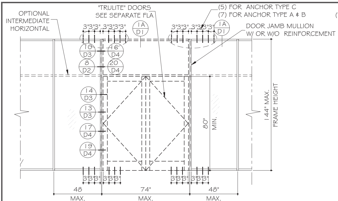
TYPICAL ELEVATION
