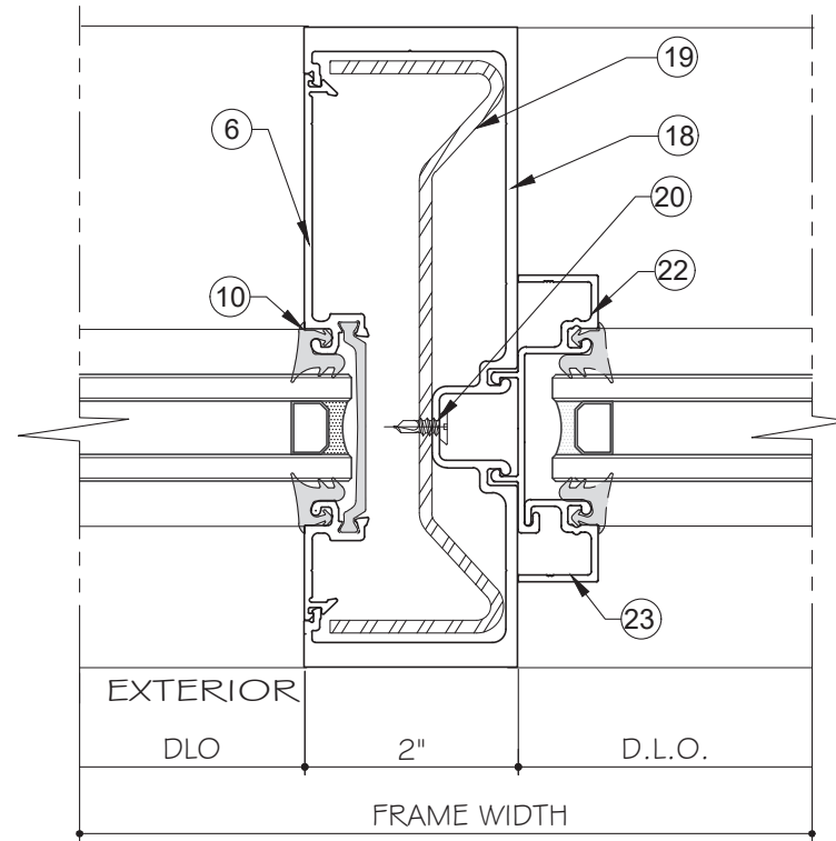
16 D4 DETAIL
