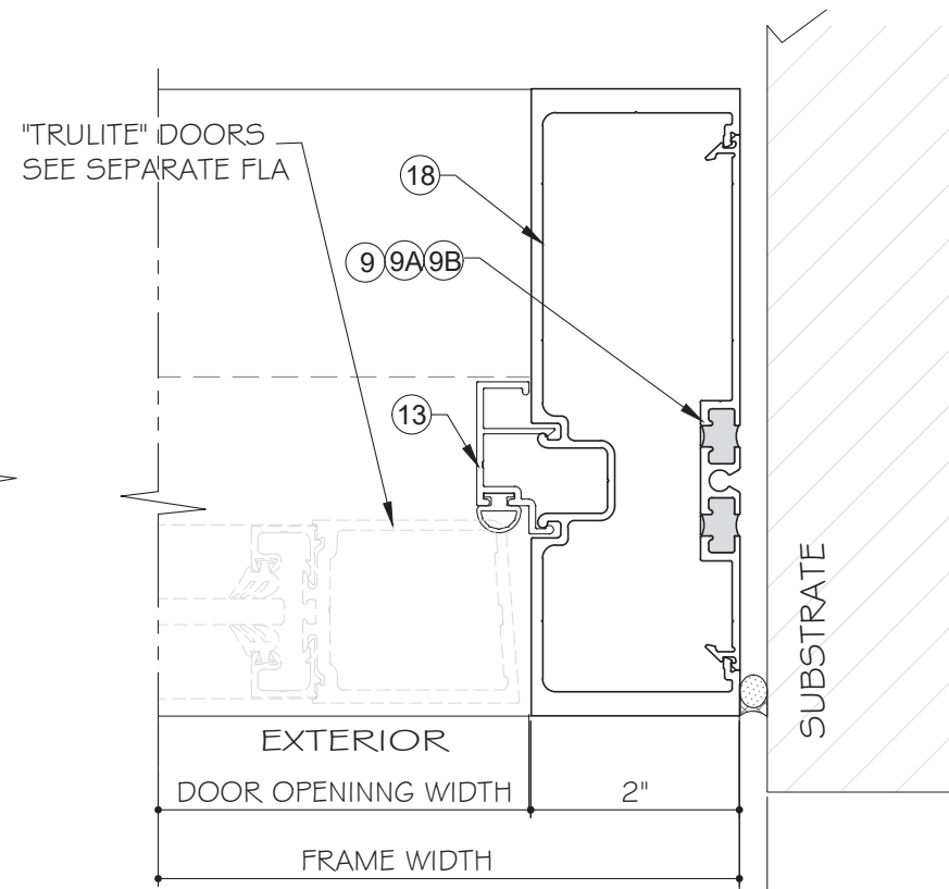
25 D4 DETAIL
