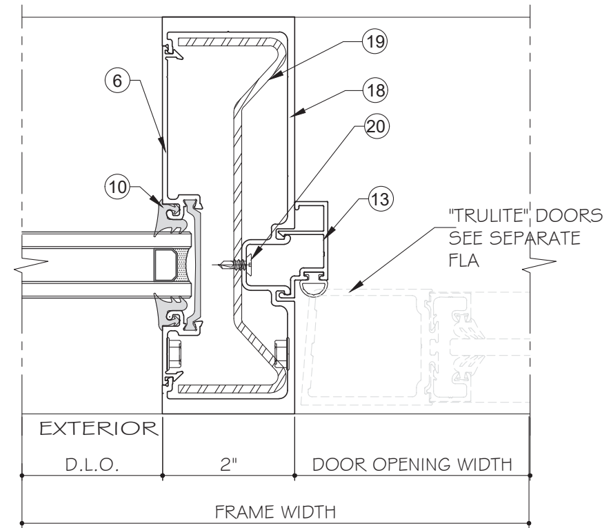
17 D4 DETAIL
