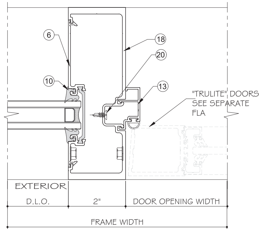
19 D4 DETAIL
