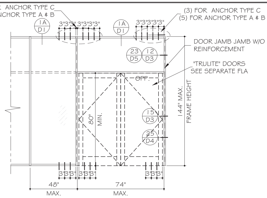
TYPICAL ELEVATION
