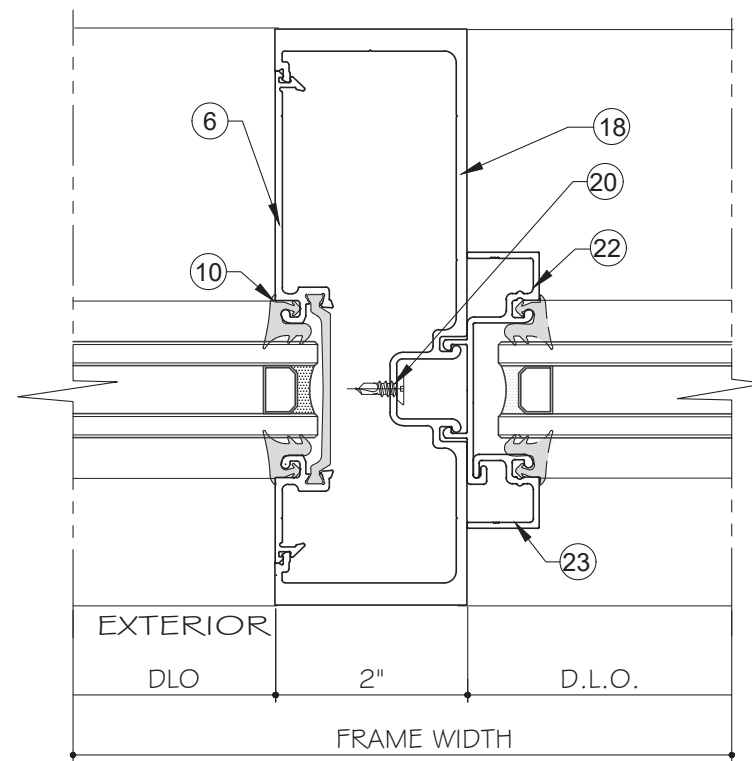
20 D4 DETAIL
