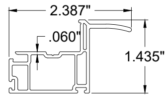
⑨ TOP PULL RAIL
