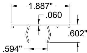
⑤ SASH ADAPTER
