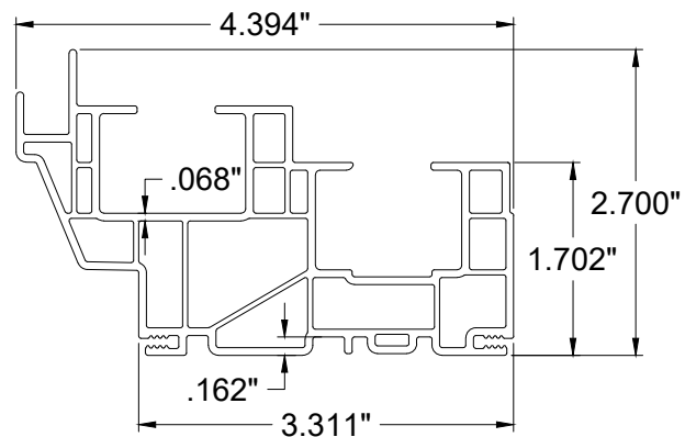
①A EQUAL-LEG FRAME
