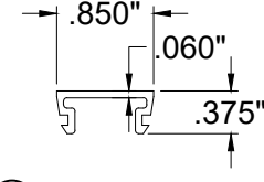
⑭ TOP PULL RAIL REINFORCEMENT
