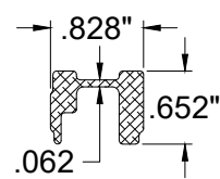
⑪ STILE REINFORCEMENT
