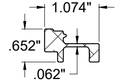
⑬ LOCK RAIL REINFORCEMENT
