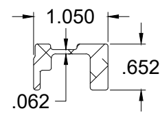
⑫ KEEPER RAIL REINFORCEMENT
