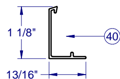
PVC MTG RAIL COVER S-6228
