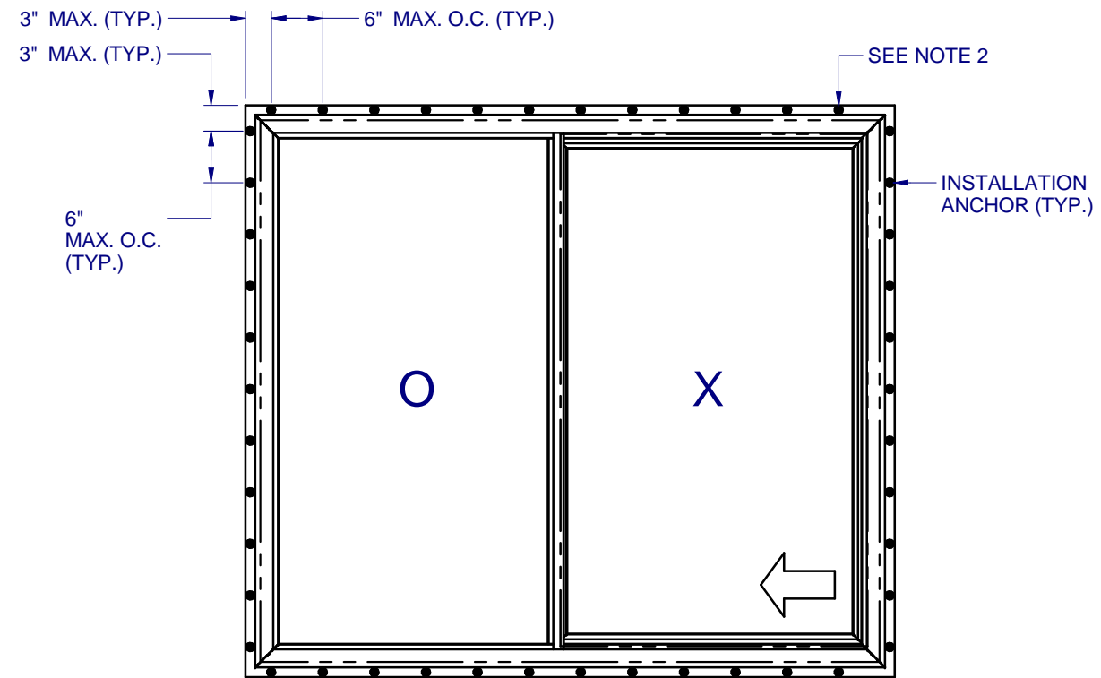
ANCHOR LAYOUT - (FIN)
