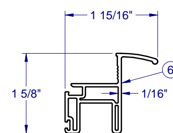
PVC SASH PULL RAIL/STILE H-6223
