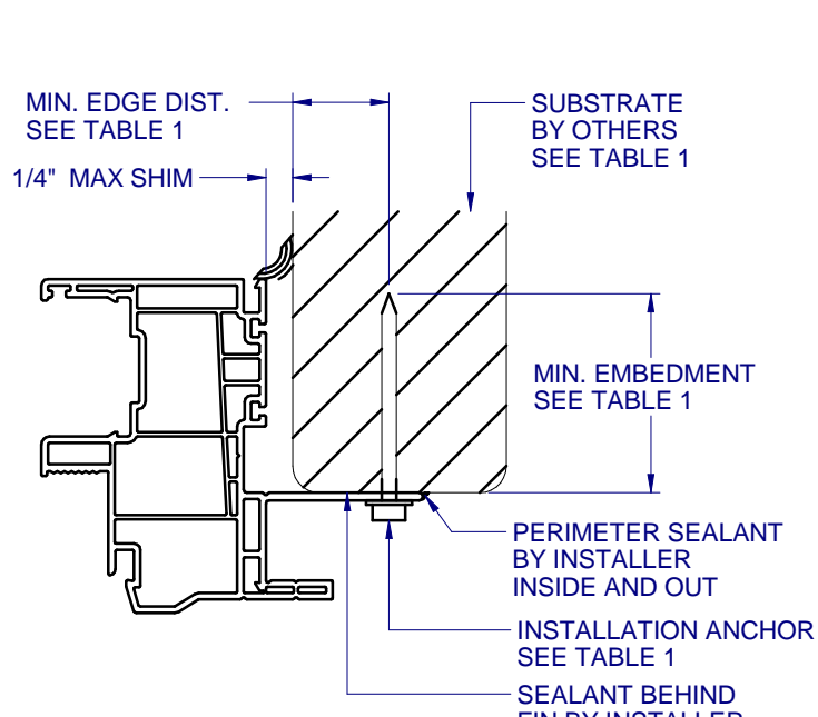
C HORIZONTAL SECTION 6 TYPICAL FIN/FLANGE ANCHORAGE HEAD AND SILL SIMILAR FOR FIN INSTALLATION
