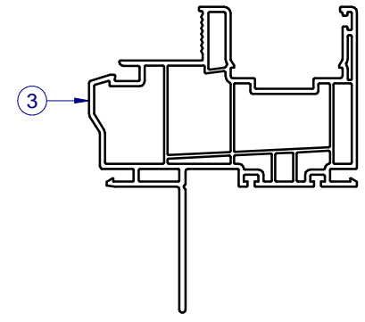
SECTION C-C ALT. FIN FRAME
