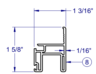
PVC SASH RAIL/STILE H-6225
