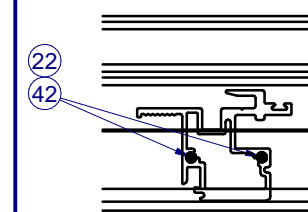
FIXED MEETING RAIL SCREWED TOGETHER WITH OUTERFRAME 1:8
