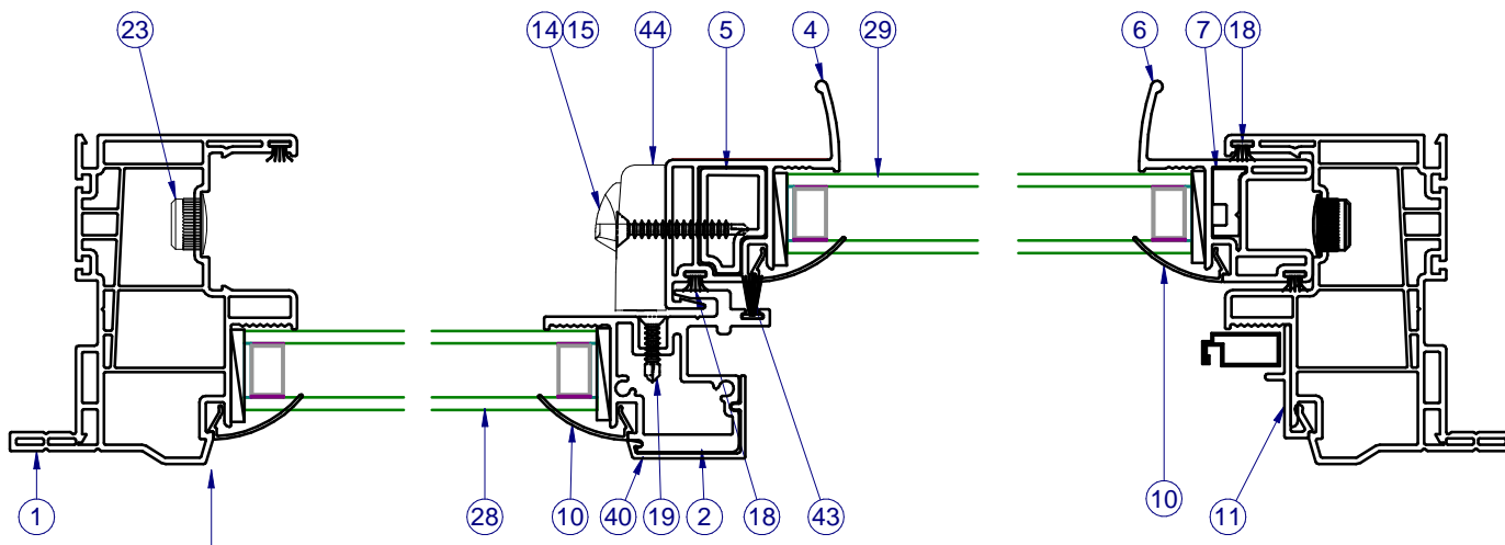
SECTION VIEW B-B NOTE: FIXED LITE AT HEAD AND SILL IS SIMILAR.
