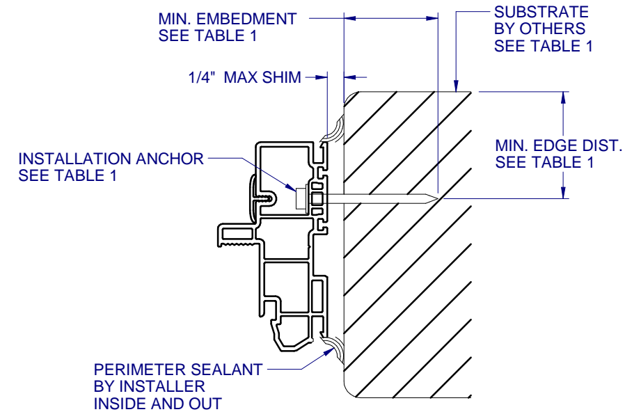
C 7 HORIZONTAL SECTION BOX FRAME INSTALLATION HEAD AND SILL SIMILAR FOR BOX INSTALLATION
